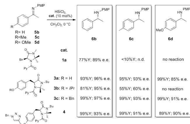
Scheme 1. Comparison of different catalytic activities 1a , 3a-3c and 4 . Reaction conditions: 5 (0.1 mmol), cat. 0.01 mmol, HSiCl 3 (0.35 mmol, 35 μL) in CH 2 Cl 2 (1 mL) at 0 °C;
