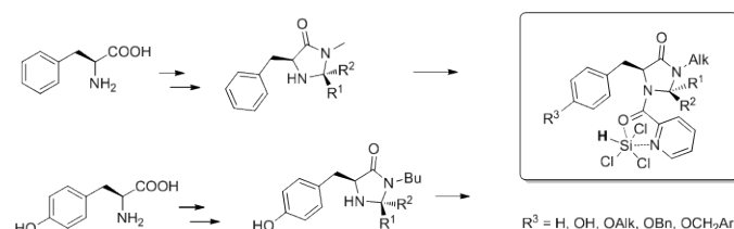
Figure 1. A new class of chiral Lewis bases for enantioselective catalytic hydrosilylation of imines.
