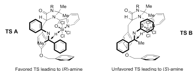
Scheme 3. Proposed TS for the reduction promoted by catalyst 3c .
