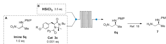
Scheme 2. Continuous flow, organocatalytic enantioselective reduction.
