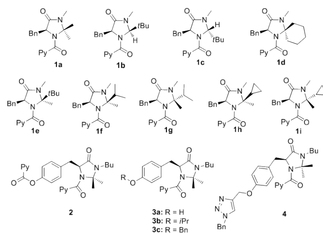
Figure 2. A new class of chiral organocatalysts for the enantioselective trichlorosilane-mediated ketoimines reduction.
