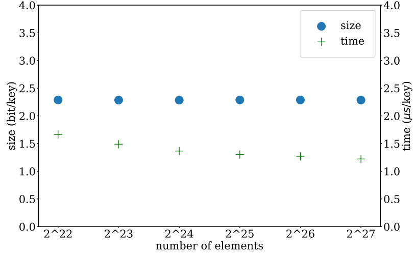
Figure 7.2: Size and construction time for increasing size of the key set (geometrically distributed output, r = 3 ).
