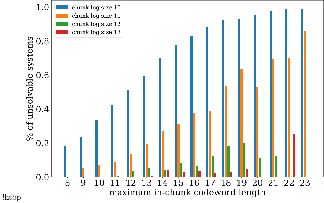
Figure 4.5: Fraction of unsolvable systems in a test dataset with geometric value distribution, k = 3 , \delta = 1.21 , depending on the maximum codeword length in the chunk.
