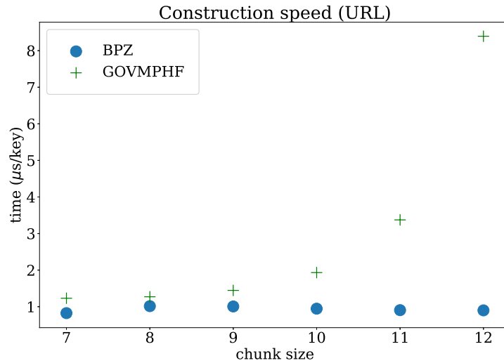
Figure 6.4: Time for BPZ and GOVMPHF on URL dataset.
