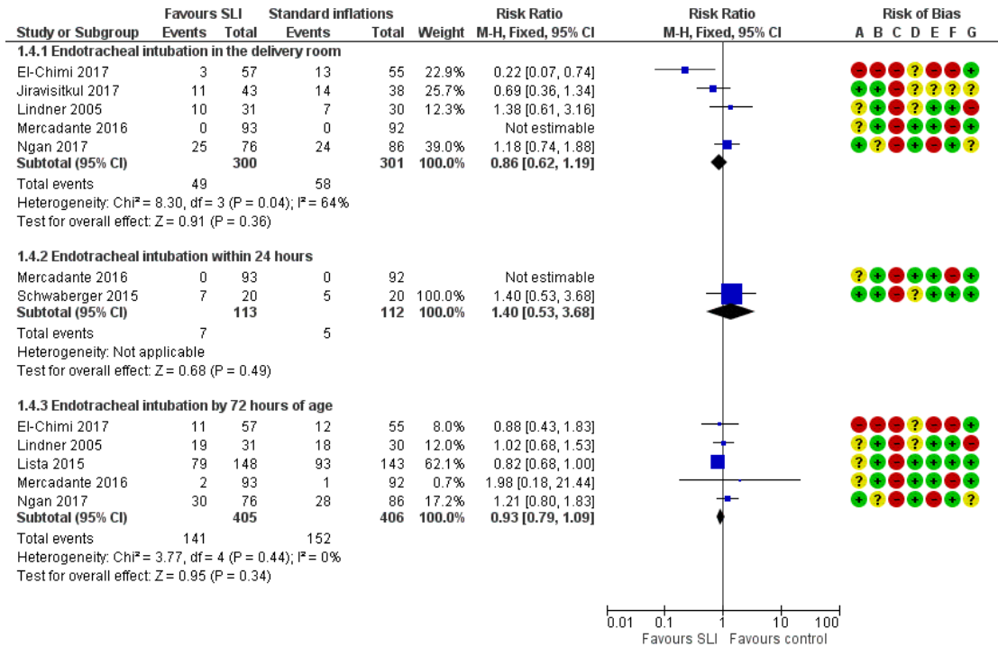
Figure 5. Forest plot of comparison: I Use of initial sustained inflation vs standard inflations in newborns receiving resuscitation with no chest compressions, outcome: I.4 Endotracheal intubation.
