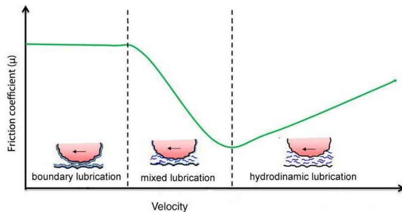
Figure 1. Schematic Stribeck curve showing coefficient of kinetic friction ( \mu ) as a function of sliding velocity in the three different lubrication regimens.
