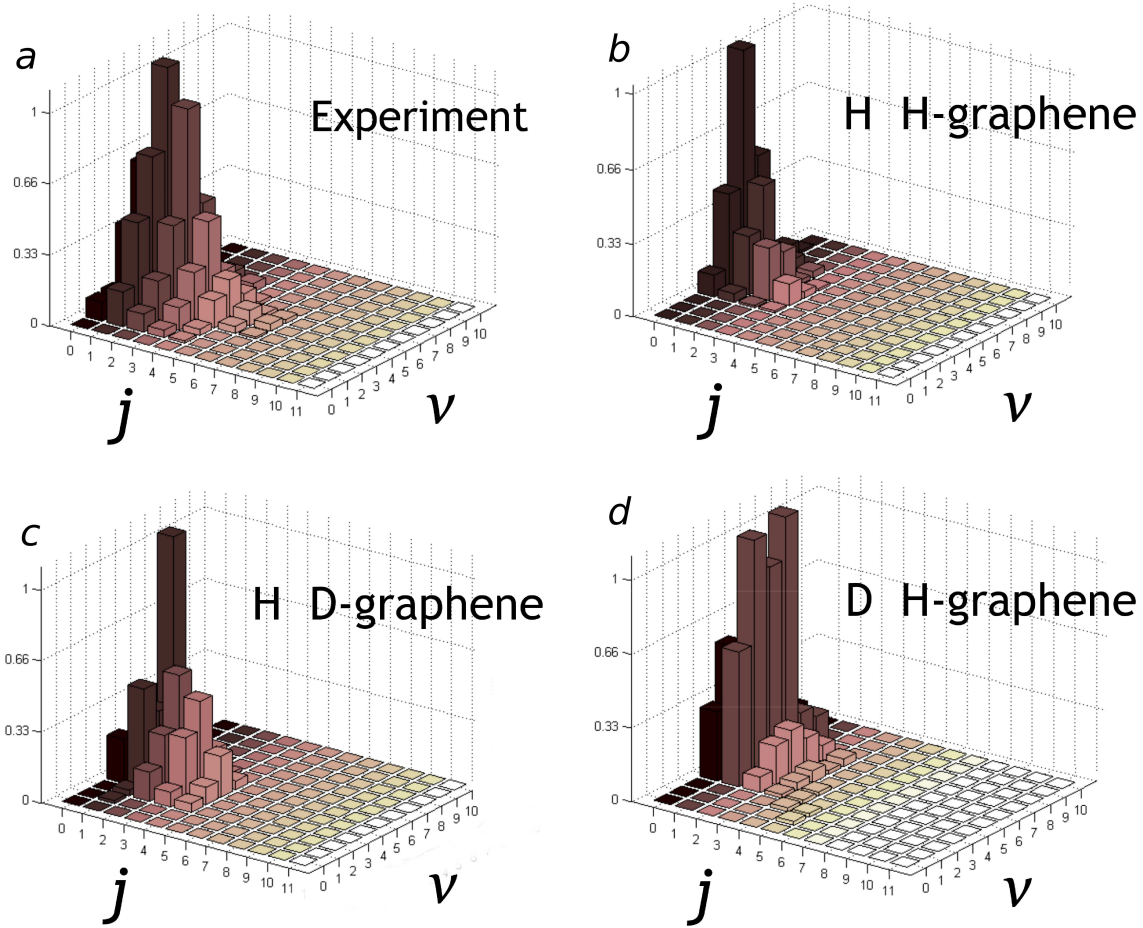
Figure 7: Relative ro-vibrational population for the product molecule. a : Experimental results from Ref. 55 for the recombination of H and D beams ( T_{gas}=300 K) on HOPG kept at T_{surf}15 K. b – d : AIMD results at E_{coll}=20 meV ( \sim 230 K) for H impinging on chemisorbed H, H on D and D on H respectively.
