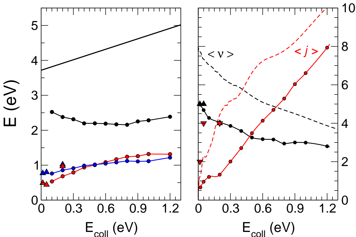
Figure 6: Left panel: Partitioning of the reaction energy into surface degrees of freedom (blue), H 2 center of mass (red) and H 2 internal (black) motion. The black line shows the total energy of the system ( \Delta H_{react} + E_{coll} ). Right panel: average H 2 vibrational (black) and rotational (red) quantum number as obtained from AIMD (dots-full lines) and quantum (dashed lines) calculations. Triangles are classical trajectory results from Ref., 44 color codes follow those of AIMD data.
