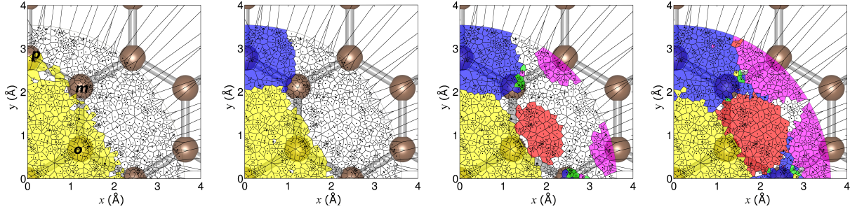
Figure 2: Aiming points location for AIMD trajectories at (from left to right) E_{coll}=0.02 , 0.2, 0.4 and 0.8 eV. The area around each aiming point was colored to match trajectories for ER (yellow), ortho dimer (red), meta dimer (green), para dimer (blue), and other dimers (magenta). The target H atom is located at the origin of the axes and the ortho (o), meta (m) and para (p) positions are indicated in the leftmost panel.
