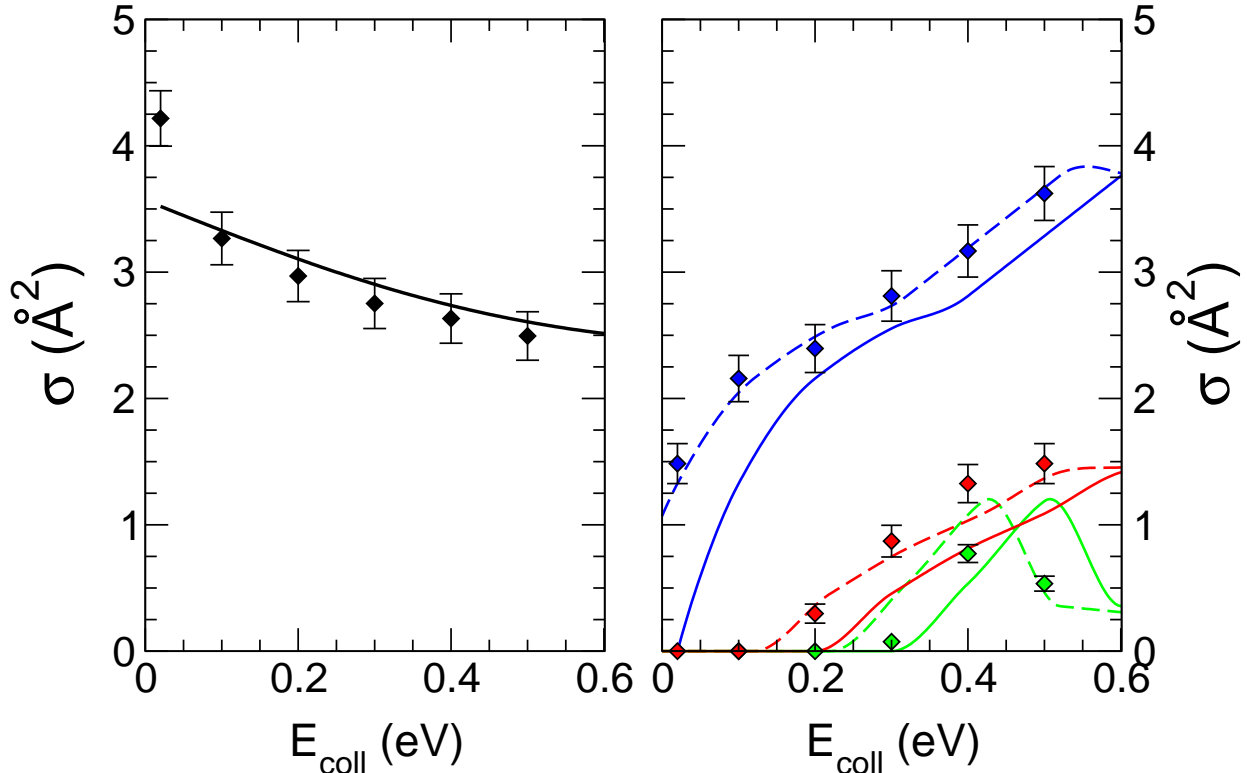
Figure 5: Effect of the van der Waals corrections to cross sections at low energies on ER (left panel) and DF (right) cross sections. Results for ER and for ortho , meta and para DF are given in black, red, green and blue, respectively. Diamonds show the vdW-corrected AIMD results, full lines show the AIMD results of Fig.1 and 4, dashed lines show the same results shifted by -80 meV.
