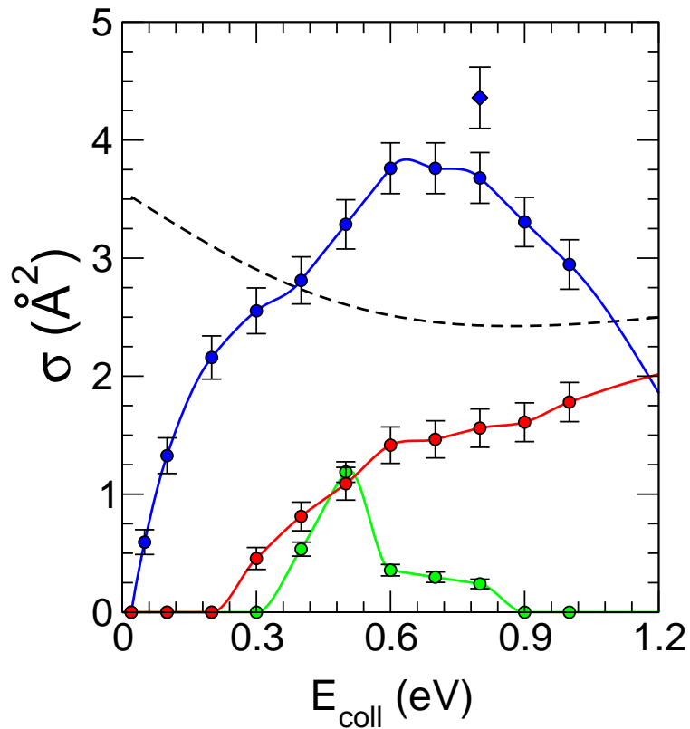
Figure 4: AIMD cross sections for the formation of H dimers: for the ortho (red), meta (green) and para (blue) dimers. The blue diamond shows the para dimer value obtained by doubling the sampled area (see text), and lines are guides to the eye. The dashed line is the ER cross section, set as a reference.
