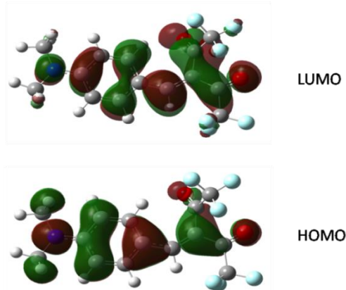
Fig. 5 Isodensity surface plot of HOMO and LUMO molecular orbitals (isosurface value 0.02).
