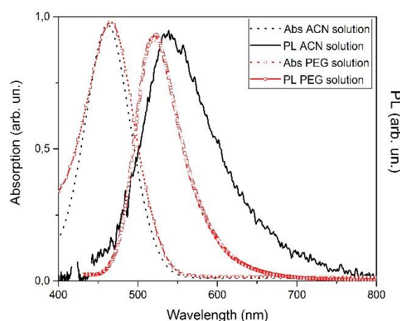
Fig. 2 Optical absorption (dashed line) and emission spectra (solid line) of 1 in ACN (black line) and PEG (red line + open squares) solutions.
