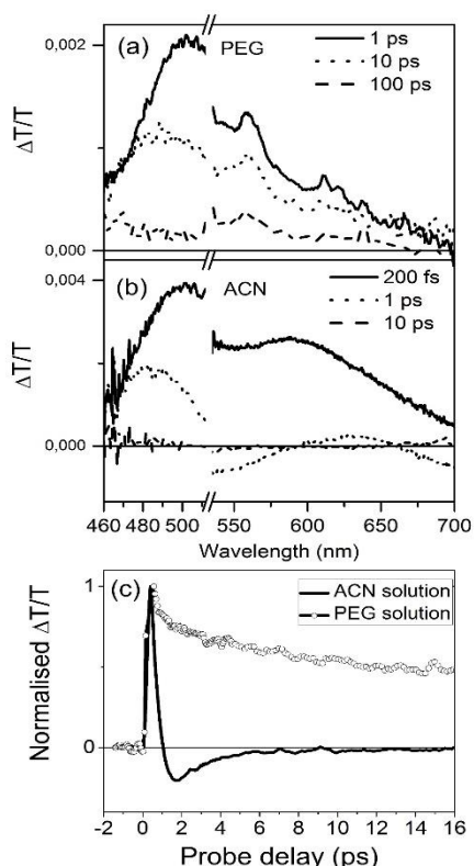
Fig. 3 \Delta T/T spectra at different probe delay for the PEG (a) and for the ACN solution (b) of 1 . Decays at 550 nm for the two solutions are shown (c)
