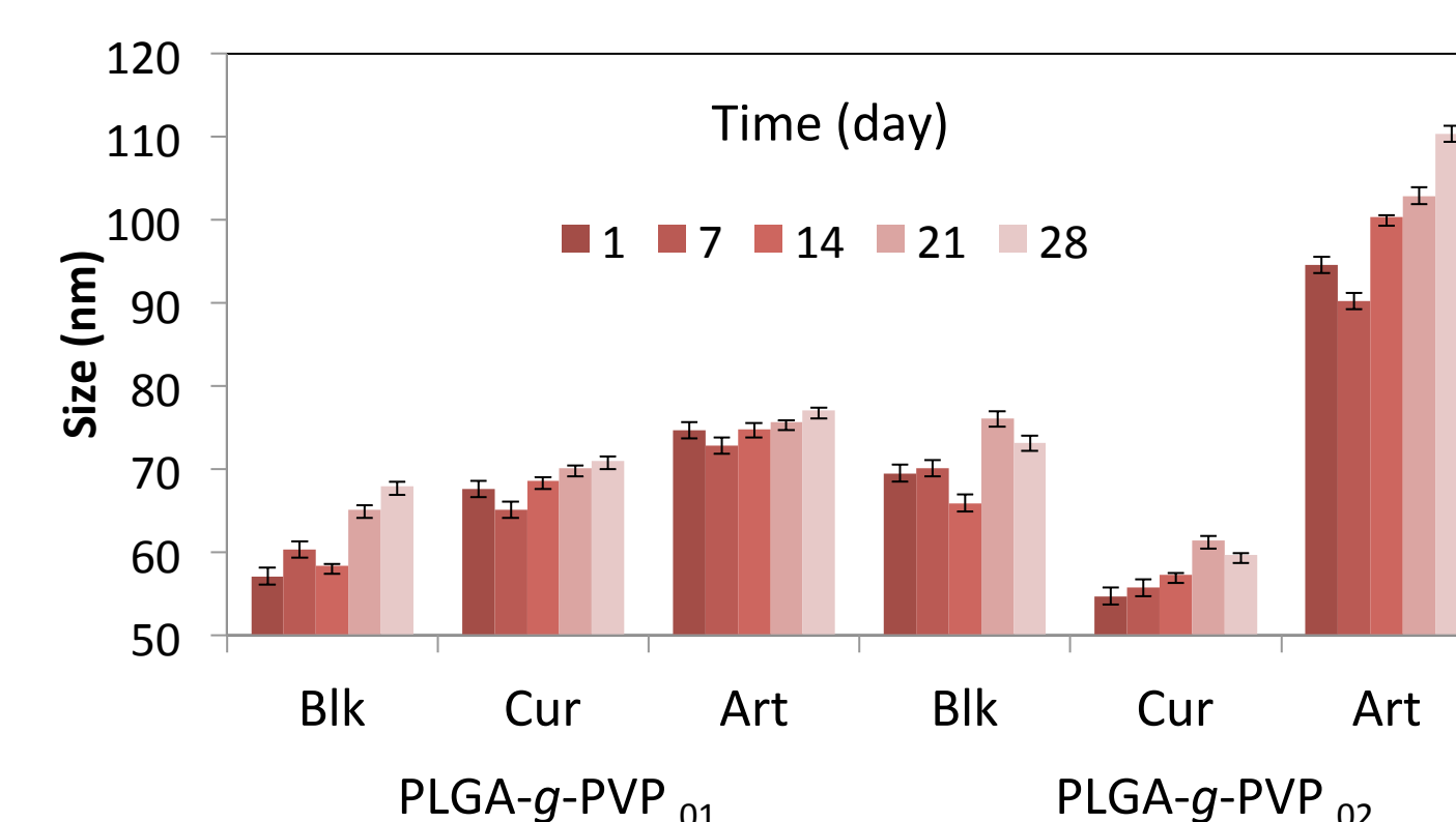
Fig. 3. Dimensional stability of unloaded and drug-loaded nanocapsules
