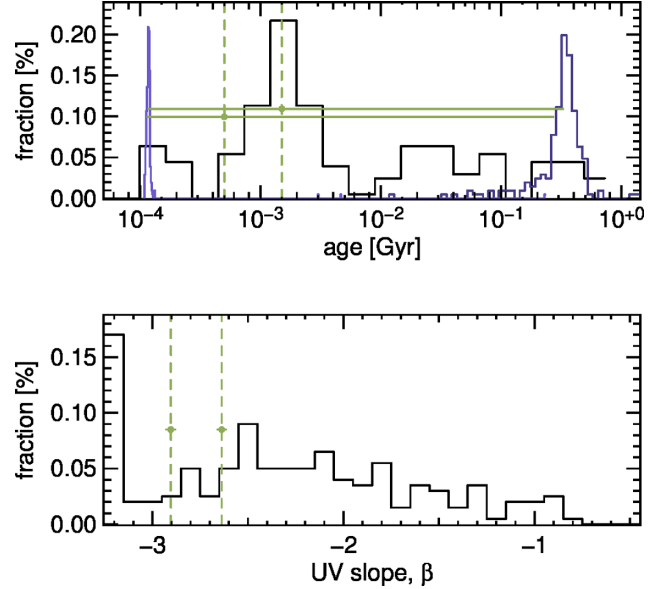
Figure 13. Upper panel: histogram of the best ages for the z \sim 6 candidates from R11, Z12 and B13 (in black). We plot in light and dark blue the age lower and upper limits, respectively, for the 2\sigma confidence level intervals of the z \sim 6 candidates. In green we plot ID2&3. The 2\sigma confidence level intervals are too large to well constrain the ages of the sources; however our multiple lensed system surely belongs to the young sample of z \sim 6 galaxies. Lower panel: histogram of the UV slope \beta as measured from the best-fitting SED templates for the B13 candidates (in black) and for our high- z galaxy (in green).
