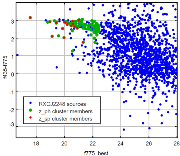
Figure 3. Colour–magnitude diagram for sources extracted in the WFC3IR FOV of RXC J2248. We plot the colour from the aperture magnitudes f435w and f775w , versus the SE extractor mag_best in the f775w filter. Blue circles are all the sources extracted in the WFC3IR FOV; red circles are the spectroscopic confirmed cluster members from Gómez et al. (2012); green circles are cluster member candidates with z_{\text{ph}} \in [0.25, 0.45] and f775w_{\text{mag\_best}} < 22.5 . We select 86 bright cluster member candidates within the 2 \times 2 arcmin 2 WFC3IR FOV, which almost all lie on the red sequence of the cluster.
