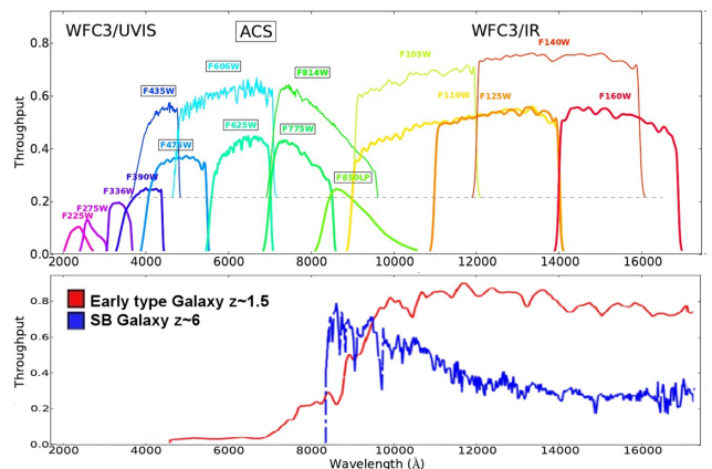
Figure 4. Upper panel: transmission curves of the HST /ACS and HST /WFC3 filters used in the CLASH survey. Lower panel: comparison of a star-forming SED redshifted to z = 6 (in blue) and an early-type galaxy at z = 1.5 (from the COSMOS library; Ilbert et al. 2009). In both cases the strong spectral break falls in the same NIR range, and both these kinds of sources appear as optical dropouts. At \lambda redder than the break the SEDs differ, thus the NIR photometry can be used to discriminate between high- and low- z dropouts.
