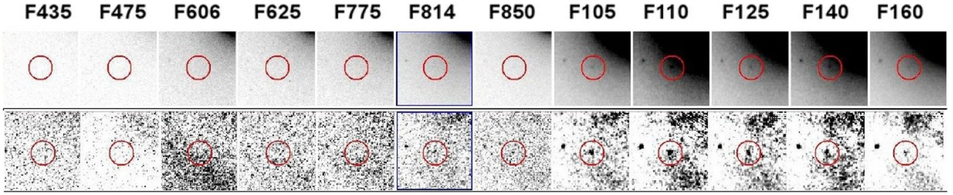
Figure 11. Postage stamps of the central image that we discover thanks to the strong lensing prediction and the subtraction of the cluster BCG. Upper panel: HST/ACS and HST/WFC3IR postage of 4 \times 4 arcsec 2 centred on the position predicted from lensing for the fifth image of the high- z system, where a source is actually observed in the NIR images. Lower panel: same as the upper panel, but for the images after the BCG subtraction: in this case there is a clear detection in the NIR filters, but also in the f814w and f850lp filters there are residuals left after the BCG subtraction.
