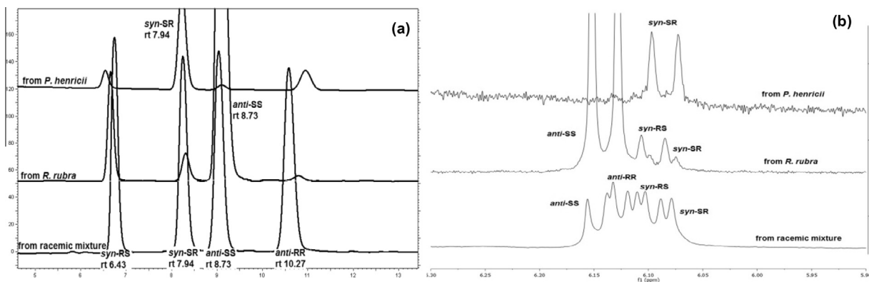
Figure 4. HPLC chromatograms for racemic mixture of 2a , reduction products from R. rubra and from P. henricii (a) compared with corresponding ^1\text{H} NMR spectra of MPA-derivatives (b).
