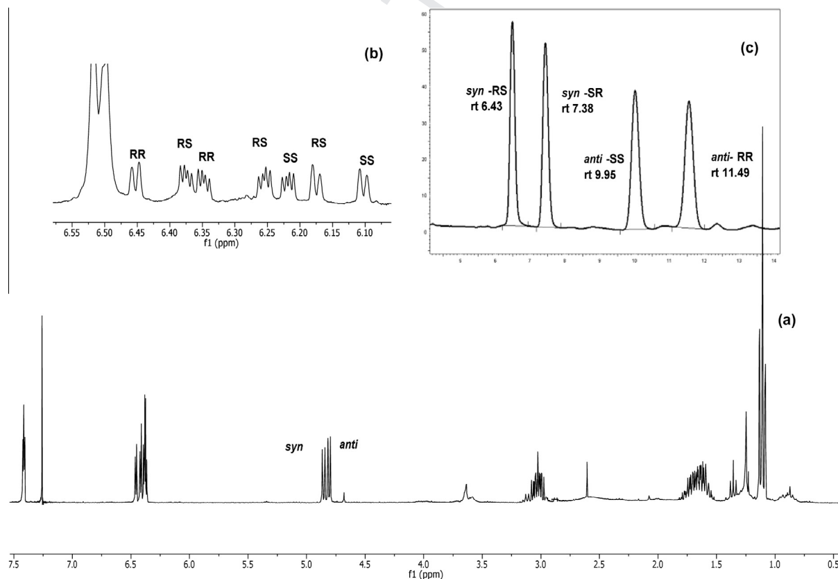
Figure 1. Comparison among 1 H NMR spectra of racemic mixture (a), S -MPA derivatives (b) and HPLC chromatogram (c) for 11a .
