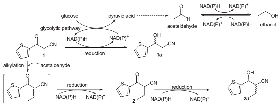
Scheme 1. Biotransformation of \beta -ketonitriles with whole-cells.
