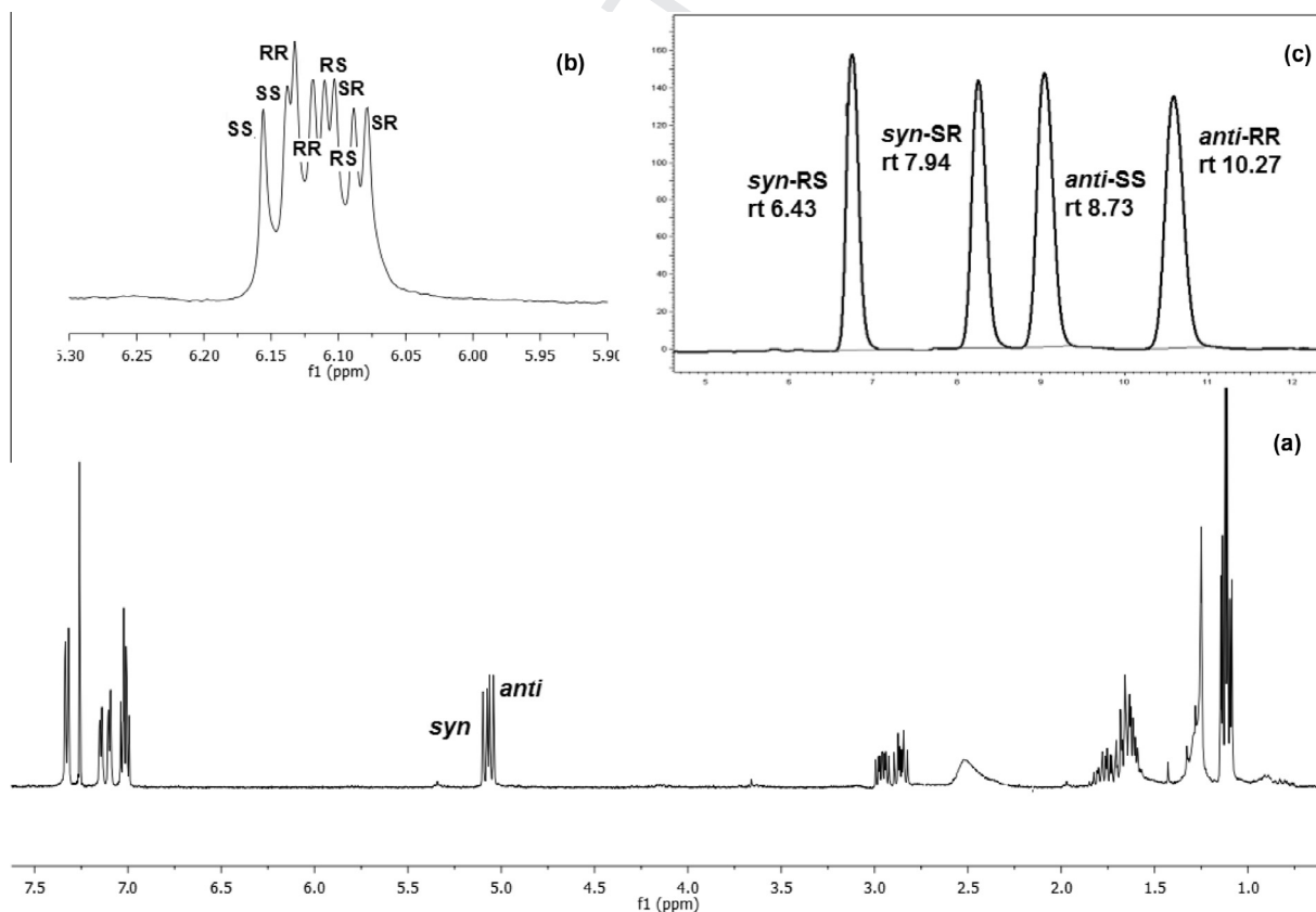
Figure 3. Comparison among ^1\text{H} NMR spectra of racemic mixture (a), derivatives with MPA (b) and HPLC chromatogram (c) for 2a .
