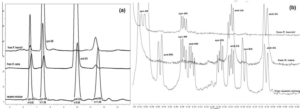
Figure 2. HPLC chromatograms for racemic mixture of 11a , reduction products from R. rubra and from P. henricii (a) compared with the corresponding ^1\text{H} NMR spectra of MPA-derivatives (b).
