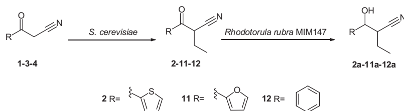
Scheme 2. Biotransformation by S. cerevisiae affording substrates 2 , 11 and 12 .
