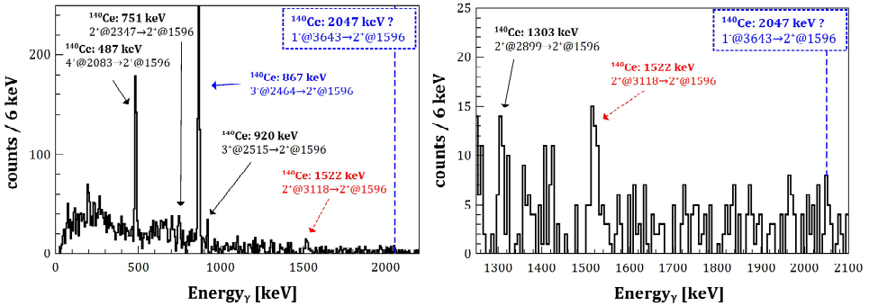
Fig. 3. Left panel: \gamma -ray energy spectrum measured in coincidence with the 1596 keV transition from the 2^+ state. Right panel: The same spectrum in the energy range from 1200 to 2100 keV. The expected energy of \gamma rays at 2047 keV is marked.
