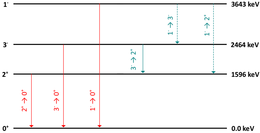
Fig. 1. Partial level scheme of ^{140}\text{Ce} showing the first quadrupole and octupole states and the candidate for the 1^- two-phonon state. \gamma transitions to the ground-state as well as the transition between phonon states are shown with solid arrows. Dashed arrows indicate the \gamma transitions from 1^- to 2^+ and 3^- constituents that were not observed yet.
