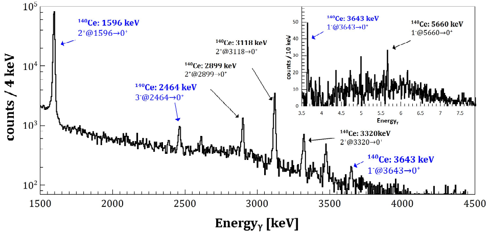
Fig. 2. A \gamma -ray energy spectrum measured with AGATA in coincidence with the ^{17}\text{O} inelastic scattering and corresponding to the selection of the ground state transitions. The transition at 3643 keV is the candidate for a de-excitation of the two-phonon state. Single-phonon 2^+ and 3^- transitions are also marked. The spectrum in PDR energy region is shown in the inset.
