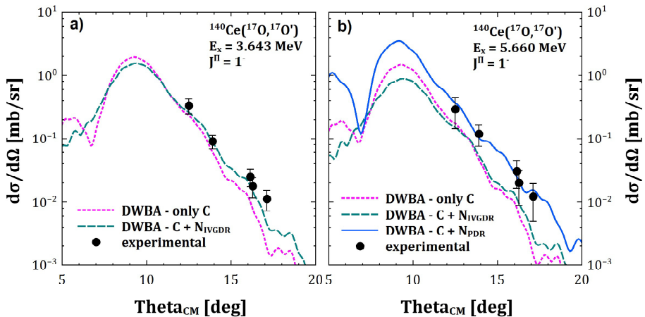
Fig. 4. Experimental cross sections for the state at 3643 keV ((a) panel) and for the state at 5660 keV ((b) panel) in ^{140}\text{Ce} measured in the present ( ^{17}\text{O} , ^{17}\text{O} ; \gamma ) experiment. The calculations shown in these panels are made using the DWBA approach. The dotted lines give the calculated Coulomb cross section (C), while the dashed lines give the total cross section (Coulomb plus nuclear contributions) and used the standard IVGDR form factor ( C+N_{\text{IVGDR}} ). The solid line represents the total cross section obtained using the microscopic form factor for pygmy states ( C+N_{\text{PDR}} ).
