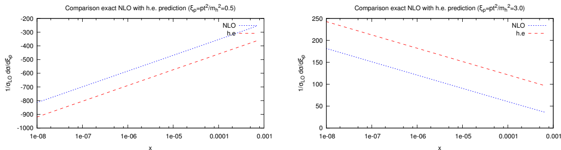
Figure 5. NLO contribution to the transverse momentum distribution for Higgs production in gluon fusion, normalized to \sigma_{\text{LO}} , compared to the high energy prediction C_2(\xi_p) eq. (4.12b) for two different fixed values of \xi_p = 0.5 and \xi_p = 3.0 .
