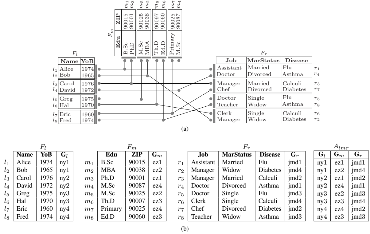
Fig. 4. Graphical representation (a) and corresponding relations (b) of a 4-loose association among three fragments F_l , F_m , and F_r of relation PATIENTS in Figure 1(a)
