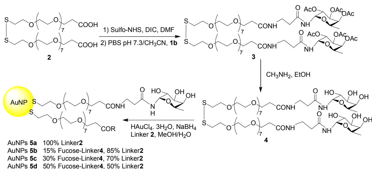
Scheme 1 Synthesis of the functionalized AuNPs 5a-d
