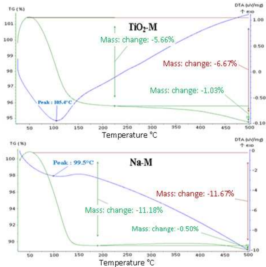
Figure 4. TG/DTA of \text{Na-M} and \text{TiO}_2\text{-M} samples
