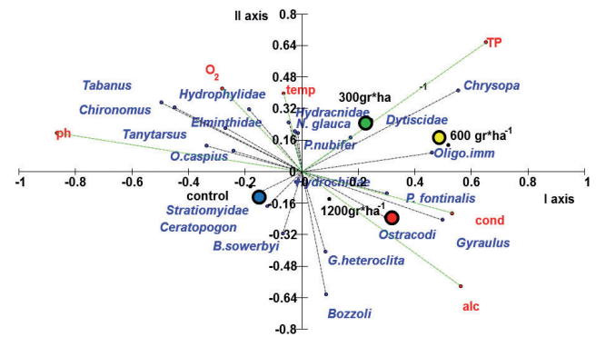
Figure 4. Canonical correlation analysis; species and environmental variables scores in the plot of the first two axes. A circle of different color maps the stations grouped according to tricyclazole treatment.
