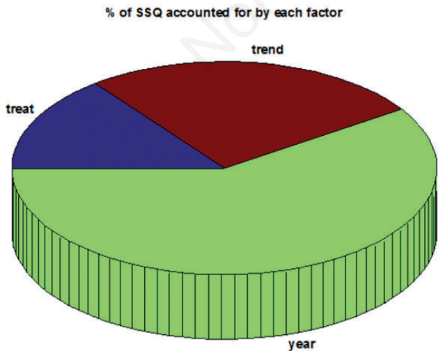
Figure 3. Proportion of sum of square (SSQ) due to different treatments; treat=SSQ bound to tricyclazole concentration, trend=SSQ bound to differences among weeks (temporal trend), year=SSQ bound to differences between years.
