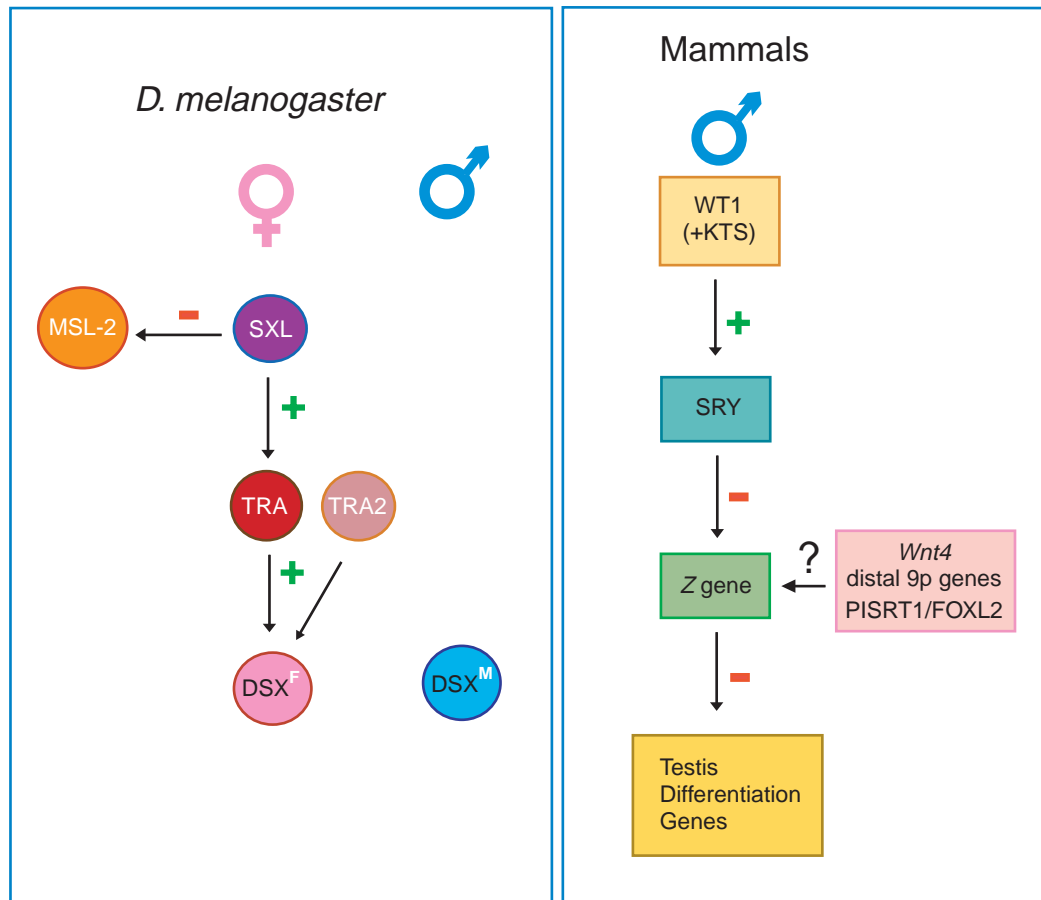
Fig. 2. Regulatory cascades in D. melanogaster and mammalian sex determination involve factors acting upon pre-mRNA splicing. In the fly (left) SXL positively regulates TRA expression and downregulates MSL-2 in female flies. TRA-TRA2 heterodimers trigger expression of the female-specific DSX F isoform. In the absence of SXL, males express DSX M . In mammals (right), WT1(+KTS) isoforms upregulate Sry in the developing male gonad. Sry, in turn, negatively influences the expression – or the function – of an unknown Z gene, which inhibits testis differentiation genes. Z gene candidates are indicated (pink box).
