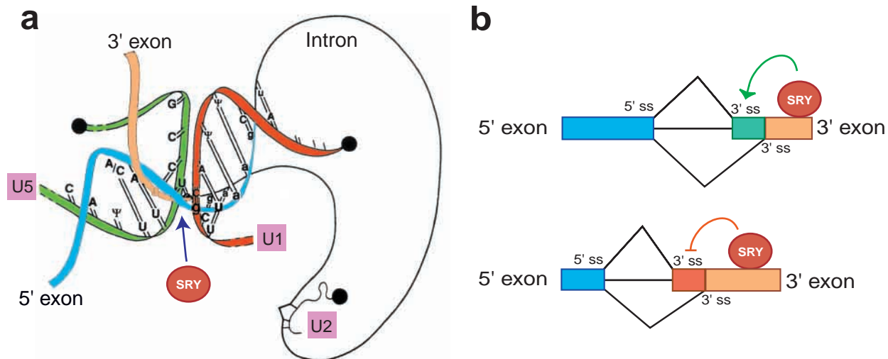
Fig. 1. Mechanisms for SRY and SOX protein function in pre-mRNA splicing. (a) Possible interaction with structures mimicking a four-way junction that favors spliceosome rearrangements during splicing (redrawn from Steitz, 1992). (b) Activation (top) or repression (bottom) of alternative splice site usage through binding to specific RNA sequences.
