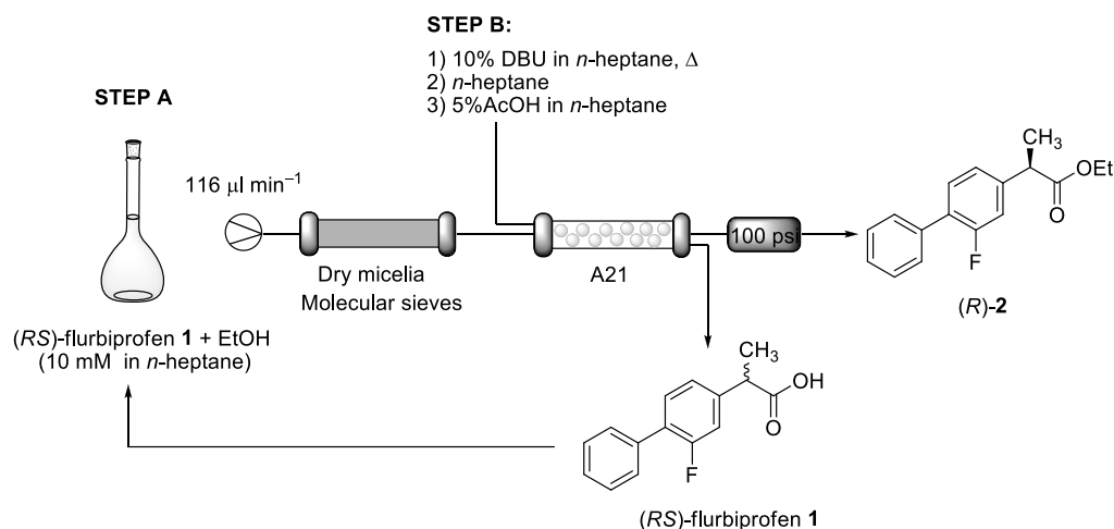
Scheme 2. Schematic representation of the overall process.
