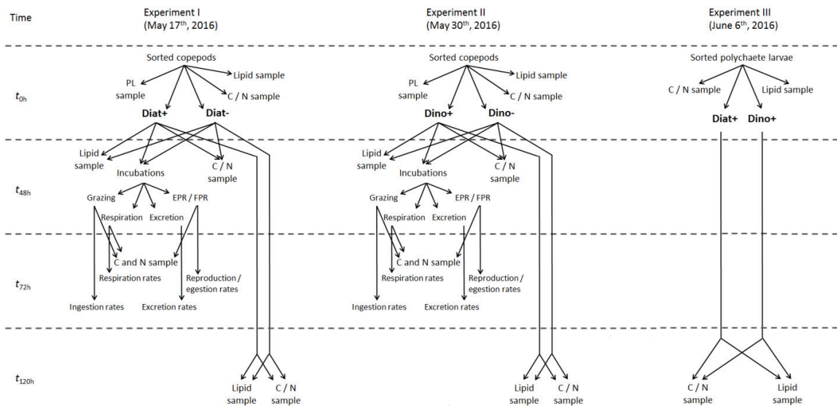
Figure 7: Experimental design used in the feeding experiments with females of the copepod Temora longicornis (Experiments I and II) and with larvae of the polychaete Lanice conchilega (Experiment III). All experiments took place immediately after zooplankton sampling. The experimental design was almost equal between Experiments I and II, except that the former was conducted with diet treatments (names in bold) consisting of diatoms cultured in nutrient-rich (Diat+) and N-limited (Diat-) conditions, whereas the latter was conducted with dinoflagellates fed with nutrient-rich (Dino+) and N-limited (Dino-) prey. Experiment III was conducted only with nutrient-rich diatom (Diat+) and dinoflagellate (Dino+) cultures. The timing of experimental phases in Experiments I and II (acclimation period, between t_{0h} and t_{48h} ; incubations, between t_{48h} and t_{72h} ; and remaining feeding time, between t_{48h} and t_{120h} ) is shown in the left column. Experiment III consisted only of feeding time (between t_{0h} and t_{120h} ). Copepods and
