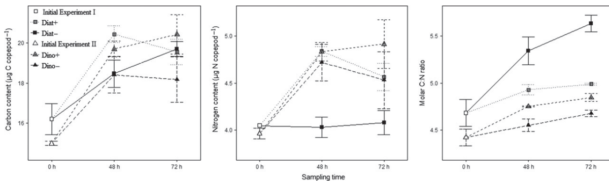
Fig. 2. C and N contents and molar C:N ratio of T. longicornis females during Experiments I and II. Experiment I tested diet treatments consisting of diatoms cultured in nutrient-rich (Diat+, gray squares and dotted lines) and N-depleted (Diat-, black squares and full lines) conditions, whereas Experiment II tested diets consisting of dinoflagellates fed with nutrient-rich (Dino+, gray triangle and dotted lines) and N-limited (Dino-, black triangle and dotted lines) prey. Samples were taken of in situ conditions ( t_{0h} , empty symbols), after 48h of acclimation ( t_{48h} ), and after 24h of incubations ( t_{72h} ). Bars represent mean values \pm one standard deviation.
