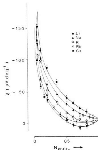
Fig. 1. Initial thermoelectric power at T=1000 K of the molten systems PbCl 2 -MeCl determined on Pb electrodes thermocells.
