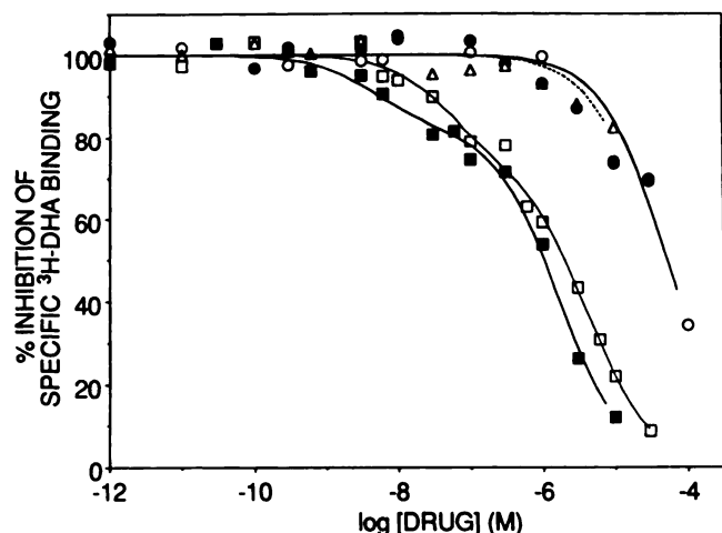
Fig. 8. Competition of serotonergic ligands for specific [ ^3\text{H} ]DHA binding in rat cerebral cortex membranes. The concentration of [ ^3\text{H} ]DHA was 2.0 nM. The data were analyzed by LIGAND, with nonspecific binding defined by 10 \mu\text{M} alprenolol. The competition curves of 8-OH-DPAT ( \Delta ), mesulergine ( \circ ), and ketanserin ( \bullet ) fit best to a single site, with their respective K_i values being 20.8, 7.2, and 17.1 \mu\text{M} . RU24969 ( \blacksquare ) and CGS-12066B ( \square ) competition curves were best fit to two sites ( p < 0.05 ). The K_i values of RU24969 for the two sites were K_{i1} = 29.4 \pm 9.0 nM and K_{i2} = 756 \pm 92 nM, whereas the K_i values of CGS-12066B were K_{i1} = 38.4 \pm 14.2 nM and K_{i2} = 576 \pm 18 nM.
