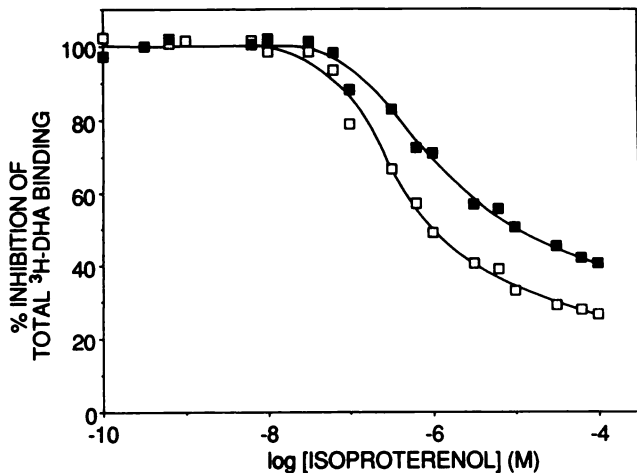
Fig. 4. Typical competition curve of isoproterenol on total [ ^3\text{H} ]DHA binding in the presence (■) or absence (□) of 300 \mu\text{M} GTP. The curves (nine experiments) were analyzed by LIGAND and nonspecific binding was defined by the program. The concentration of [ ^3\text{H} ]DHA was 2.0 nM. Specific binding was 70% of total in the absence of GTP and 57% in the presence of GTP. The competition curves of isoproterenol on [ ^3\text{H} ]DHA binding in the absence of GTP were best fit to a two-site model ( p < 0.01 ) with K_{i1} = 50.0 \pm 3.7 nM and K_{i2} = 7.18 \pm 1.79 \mu\text{M} . The capacities of the two sites (fmol/mg of tissue) were R_H = 4.56 \pm 0.32 and R_L = 6.38 \pm 0.72 . These parameters were obtained by fixing the affinity of [ ^3\text{H} ]DHA for the high affinity site at 0.6 nM while its affinity for the second site was set at 6.64 nM (the value obtained from alprenolol competition curves). The competition curves in the presence of GTP were best fit to a one-site model, with K_i = 174.5 \pm 10.0 nM ( p < 0.01 versus K_{i1} of isoproterenol in the absence of GTP) and a density of 5.26 \pm 0.46 fmol/mg of tissue.
