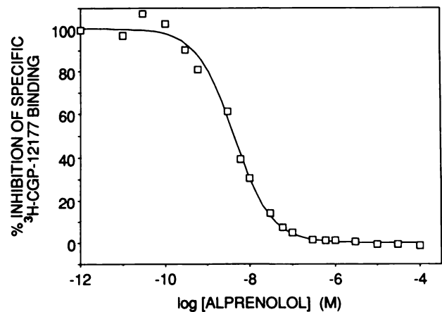
Fig. 5. Typical competition curve of alprenolol for [ ^3\text{H} ]CGP-12177 binding in rat cerebral cortex membranes. Alprenolol competition curves for 0.2 nM [ ^3\text{H} ]CGP-12177 were monophasic, with a K_i = 1.80 \pm 0.16 nM and a B_{\text{max}} = 5.16 \pm 0.14 fmol/mg of tissue (mean \pm SE of five separate competition experiments). Nonspecific binding was defined by LIGAND and amounted to 8% of total binding.
