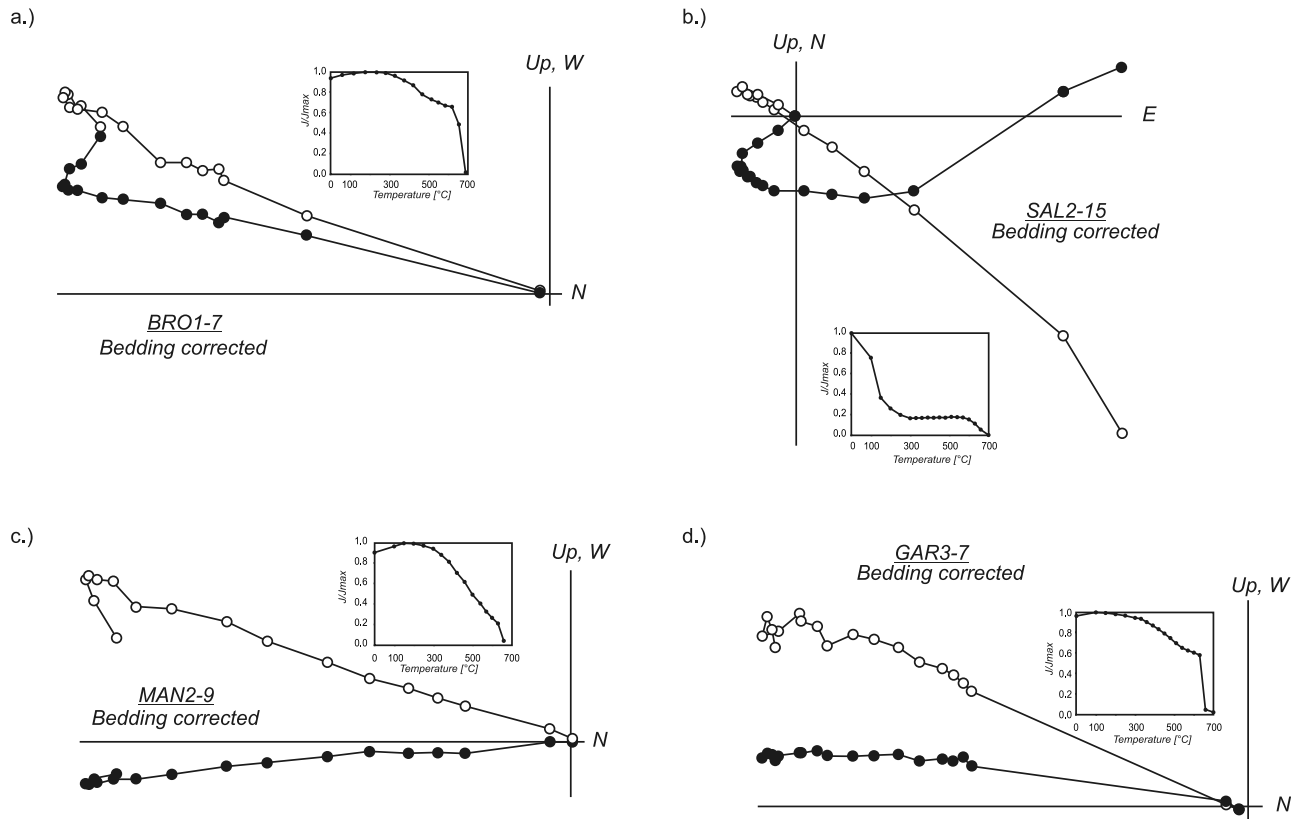
Figure 6. (a–d) Results of thermal demagnetization experiments plotted as orthogonal vector diagrams [Zijderveld, 1967] in stratigraphic coordinates together with normalized diagrams of intensity decay. Full (open) dots represent vector endpoints projected onto the horizontal (vertical) plane. For clarity NRM values are not plotted.
