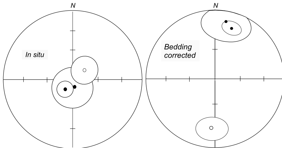
Figure 9. Stereographic projections of all Triassic site mean directions in in situ and bedding corrected coordinates. Open (closed) symbols indicate negative (positive) inclinations.
