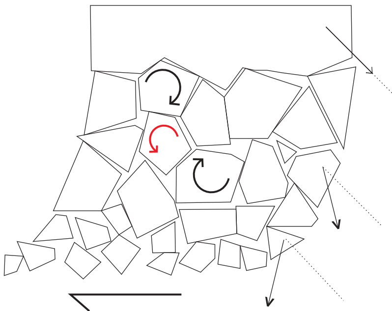
Figure 12. The small block model as proposed by McKenzie and Jackson [1983]. The brittle upper crust is broken into small blocks which rotate in response to the continuous, ductile deformation at greater depth. Notice the interaction between single blocks. Redrawn and modified after Nelson and Jones [1987]. Small black arrows on the right represent the direction of an ancient magnetization direction.
