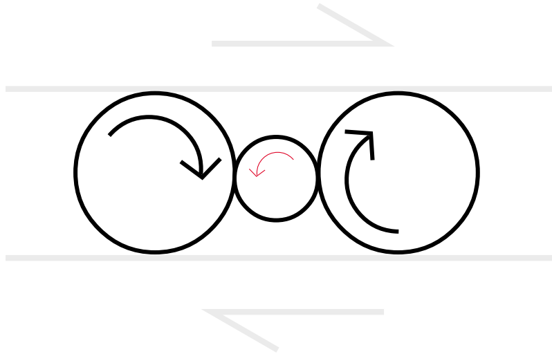
Figure 11. Simple ball bearing model to explain the observed differential rotations.
