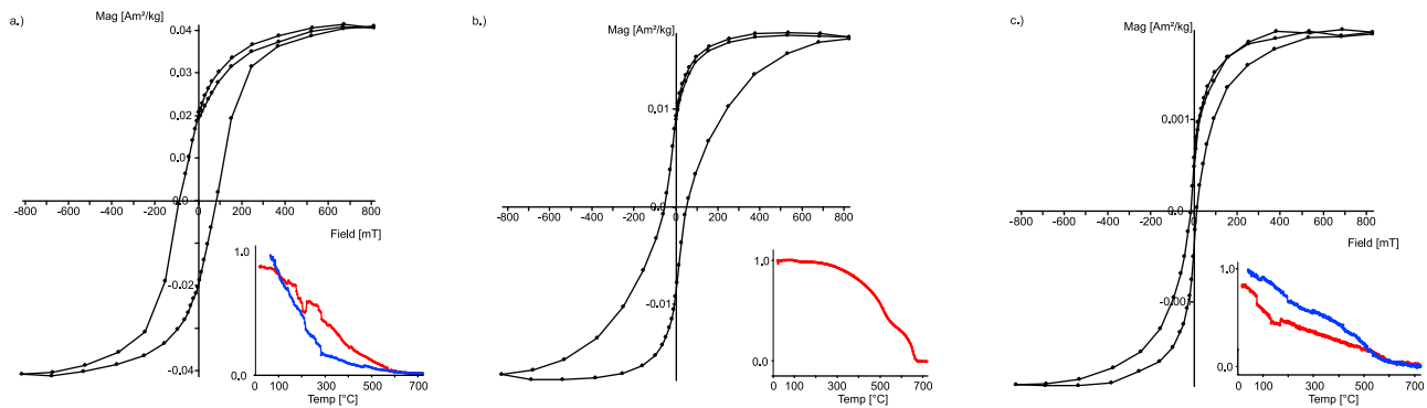
Figure 5. Hysteresis curve for (a) one of the Les Salettes tuff samples, (b) one of the Saint-Mandrier tuff samples and (c) one of the Saint-Mandrier redbed samples. The thermomagnetic curves are plotted with normalized intensities.
