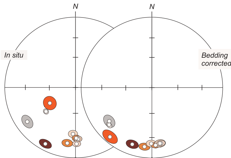
Figure 8. Stereographic projections of all Permian site mean directions in in situ and bedding corrected coordinates. Open symbols indicate negative inclinations.
