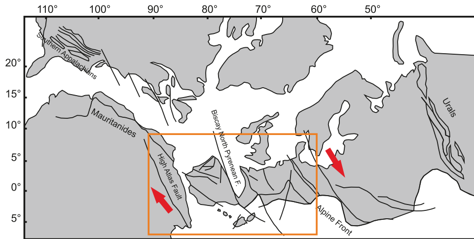
Figure 1. Location and outlines of the Pangea Transform Zone after Arthaud and Matte [1977].
