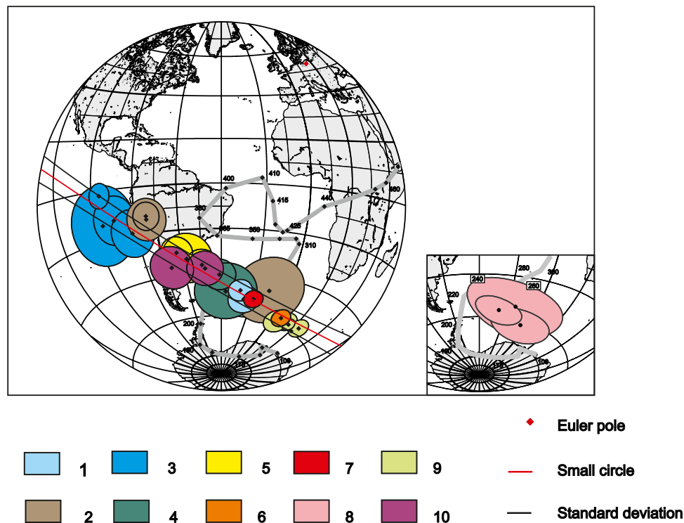
Figure 10. 1–5: Virtual geomagnetic poles from previous studies (Tables 2 and 3); 6–10: Virtual geomagnetic poles from this study (Table 1) with respect to the apparent polar wander path of Baltica [Smethurst et al. , 1998]. The poles plot on a small circle about a Euler pole in present-day northwest Europe. Legend: (1) Estérel, (2) Maures, (3) N Corsica, (4) NW Sardinia, (5) S. Corsica–N. Sardinia, (6) BAR, (7) BRO, (8) GAR, (9) MAN, (10) SAL. The inset shows the three Triassic virtual geomagnetic poles from this study (calculated from paleomagnetic mean directions from sites GAR1, GAR2 and GAR3).
