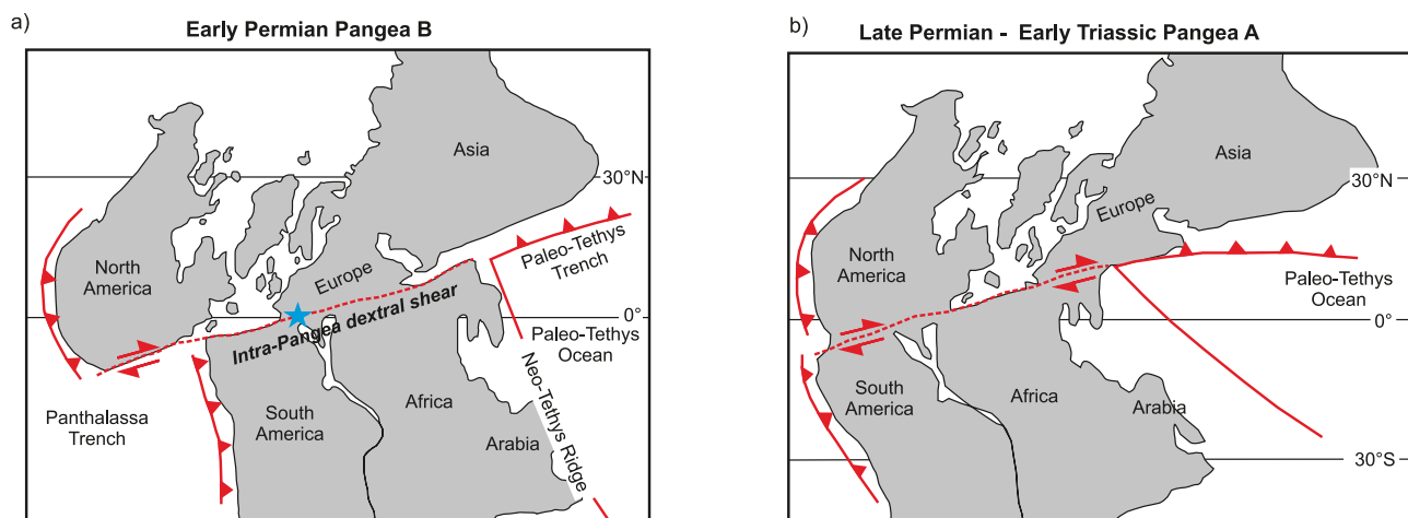
Figure 2. (a) Pangea B configuration after Irving [1977] in the Early Permian. (b) Wegenerian Pangea A configuration after Muttoni et al. [2003, 2004] in the Late Permian to Early Triassic. The blue star marks the study location in SW Europe. Modified after Muttoni et al. [2009].
