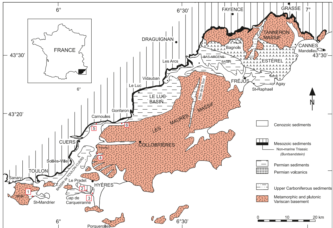
Figure 3. Geological outline of Provence, SE France including sample locations: (1) five sites within the Saint-Mandrier Fm., (2) three sites within the Grès de Gonfaron (sandstone), (3) three sites within the Les Salettes Fm., (4) sites within the LesPellegrins Fm. (rejected from the data set), (5) one site within the Bron Fm. near Carnoules, and (6) two sites within the Bron Fm. near Saint Barthélémy. From Cassinis et al. [2003], modified and redrawn.
