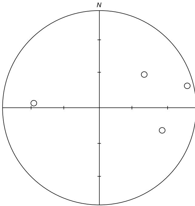
Figure 7. Paleomagnetic results based on four samples from a polymictic conglomerate from the Les Salettes Formation show a widely distributed directional data set which might be taken as evidence for a primary age of magnetization. Open symbols indicate negative inclinations.
