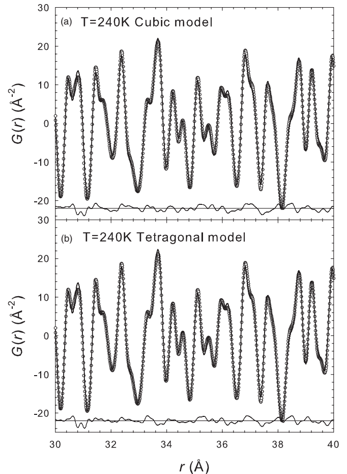
FIG. 9. Observed (dots) and calculated (continuous lines) high- r PDF for \text{EuTiO}_3 at 240 K. (a) and (b) are the fits obtained using the cubic average model and low-temperature tetragonal model, respectively.
