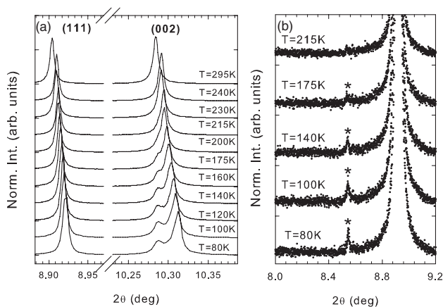
FIG. 1. Selected 2\theta regions of \text{EuTiO}_3 x-ray diffraction patterns are shown as a function of temperature. (a) The temperature evolution of the Miller index (111) and (002) peaks related to the room-temperature cubic phase. (b) The appearance of a weak superlattice reflection as a function of temperature.
