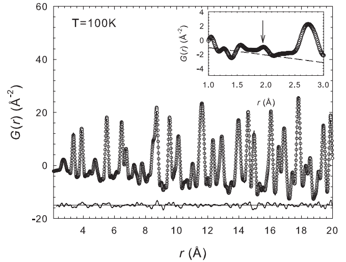
FIG. 7. Observed (dots) and calculated (continuous line) PDF obtained for \text{EuTiO}_3 at 100 K. The residual plot is shown at the bottom of the figure. In the inset, a region of short interatomic distances is displayed. The dashed line is the baseline and corresponds to -4\pi r\rho_0 [see Eq. (1)]. The arrow indicates approximately the r position of Ti-O interatomic distances.
