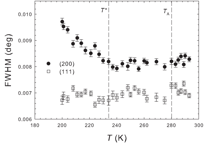
FIG. 6. Temperature evolution of the (200) and (111) Bragg families FWHM for the cubic phase of \text{EuTiO}_3 .
