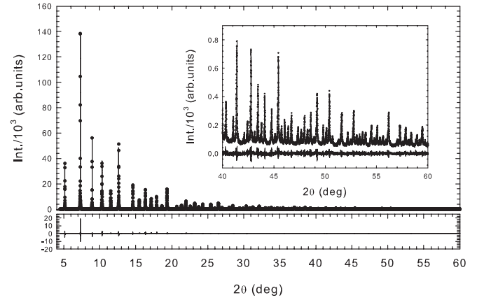
FIG. 3. Measured (dots) and calculated (lines) powder-diffraction patterns for \text{EuTiO}_3 at 100 K. The inset shows a magnified view of the high-angle diffraction peaks. The difference between the observed and fitted patterns is displayed at the bottom of each figure.
