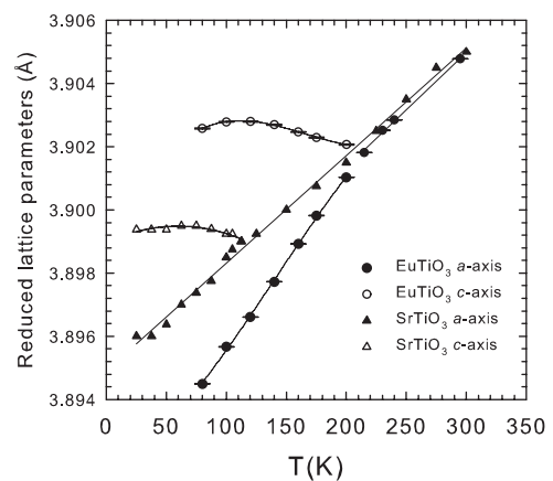
FIG. 2. Reduced lattice parameters of \text{EuTiO}_3 and \text{SrTiO}_3 as a function of temperature. The full and opened circles are the a and c axes of \text{EuTiO}_3 . Full and opened triangles indicate the a - and c -axis values of \text{SrTiO}_3 derived from Ref. 21. The continuous lines are guides to the eye.
