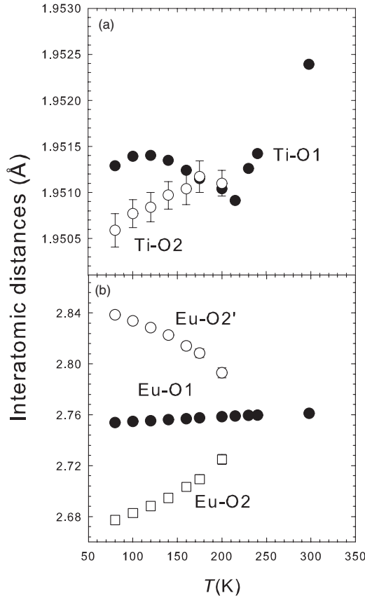
FIG. 4. (a), (b) The refined Ti-O and Eu-O interatomic distances as a function of temperature.
