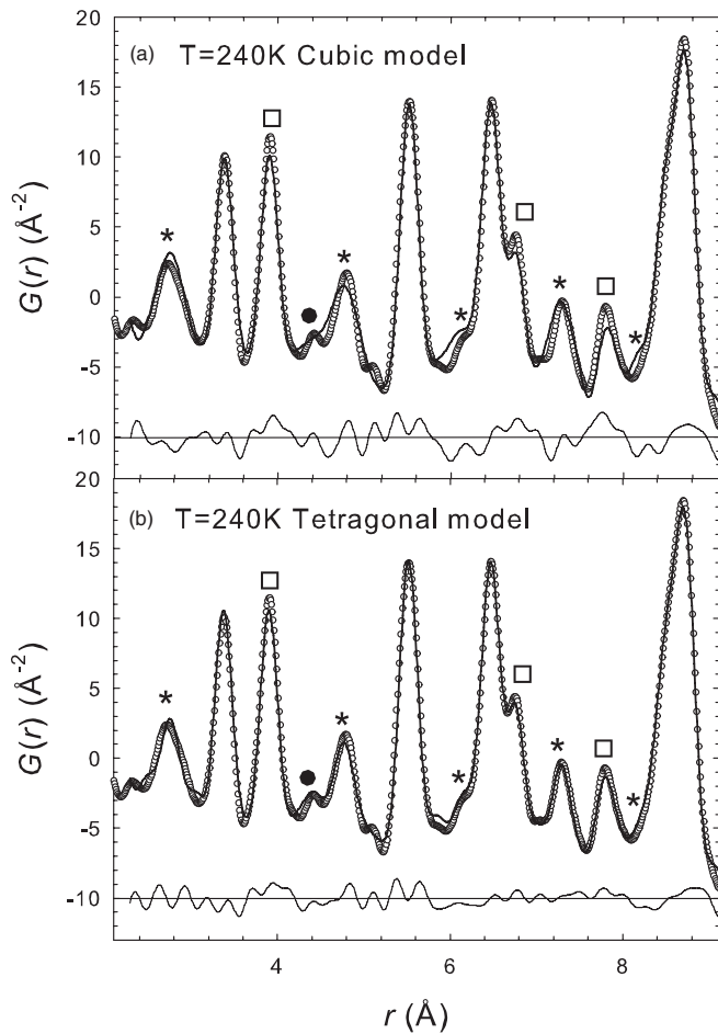
FIG. 8. Short-range observed (dots) and calculated (continuous lines) PDF for \text{EuTiO}_3 at 240 K. (a) and (b) are the fits obtained using the cubic average model and the low-temperature tetragonal model, respectively. The symbols in the panel label the PDF peaks belonging to Eu-O (stars), Eu-Eu (empty squares), and Ti-O (full circles) interatomic distances.
