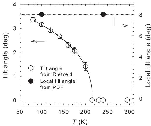
FIG. 5. \text{EuTiO}_3 octahedral tilting angle values (empty circles) as a function of temperature obtained from the Rietveld refinement (Table I). The continuous line is the best fit for the critical equation \phi_-(T) = \phi_-(0)(1 - T/T_c)^\beta , by setting T_c = 215 K. The full circles are the tilting angle values obtained from PDF refinements (Table II).
