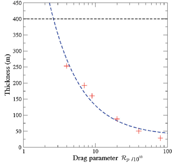
Figure 4. We plot the extent of the region in which Kelvin oscillations can be excited as a function of the weak drag parameter \mathcal{R}_p . Note that the whole strong pinning region is 400 m thick, as indicated by the horizontal line. We extrapolate the value of the drag parameter for which the whole region is involved by fitting a function of the form, inspired by the estimate in (21), f(x) = a + b/(\mathcal{R}_p/10^{-10}) , where the best-fitting parameters were a = 34.77 \pm 13.7 \text{ m} and b = 955.8 \pm 101.9 \text{ m} . As we can see, the whole strong pinning region participates in the glitch for \mathcal{R}_p < 2 \times 10^{-10} , as expected from the analytical estimates.
