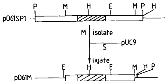
Figure 1. The plasmid pO61M was constructed by restriction enzyme digestion of pO61SP1 with Mn I, isolating the 1304 bp fragment containing the ogt gene and ligating this into Sma I digested pUC9. Resultant clones were analysed by digestion with Eco RI or Hind III. E, Eco RI; H, Hind III; M, Mn I; P, Pst I; S, Sma I.
