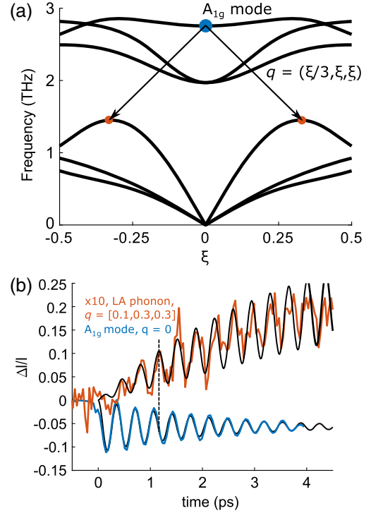
FIG. 1. (a) Phonon dispersion relation in bismuth along the q = (\frac{1}{3}\xi \xi \xi) direction, illustrating a decay channel of an A_{1g} phonon into a pair of LA phonons at q and -q . (b) experimental signature of decay of the A_{1g} phonon in bismuth by the channel shown in (a). The lower (blue) curve shows the relative intensity change of the (2 3 2) Bragg peak, which is proportional to the A_{1g} mode amplitude. The upper (orange) curve shows the relative intensity change of the diffuse scattering \Delta I/I in a region near q = (0.1 \ 0.3 \ 0.3) in the (0 1 1) zone (multiplied by 10). The black lines are simulations. The dashed line indicates a \pi/2 phase shift between the A_{1g} mode and the target mode.
