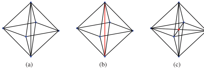
Fig. 6.5: The bisection of four tetrahedrons. a) Four tetrahedrons; b) The refinement edge (in red); c) Eight tetrahedrons, with the new vertex (in red).
