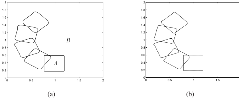
Fig. 4.6: Tracking of a square with (a) 10000 degrees of freedom and cfI = \frac{1}{10} and (b) 40000 degrees of freedom and cfI = \frac{1}{10} .
