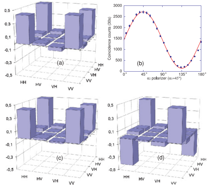
FIG. 4. (Color online) Characterization of the output state. In (a) we report the tomographic reconstruction (real part) of the global purified polarization entangled state prior to the action of the phase gate, whereas in (b) we show the corresponding visibility curve and the fit with the curve \cos^2(\alpha - 45^\circ) (solid line). In (c) and (d) we report the tomographic reconstructions (real part) of the reduced states q_0 and q_1 .
