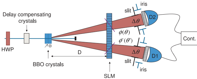
FIG. 2. (Color online) Experimental setup. Polarization entangled states are generated by down-conversion in type-I BBO crystals pumped at 405 nm by a Newport LQC 405-40P cw laser diode. Then, a spatial section of the output cones passes through the SLM which (at the same time) i) provides purification of polarization entanglement and ii) introduces a position- (i.e., generation angle) dependent phase shift between the two polarizations. After SLM, there are (on both paths) a slit, an iris, two long-pass filters (cut-on wavelength = 715 nm), a coupler with an 1/e^2 output beam diameter of 7.14 mm, and a multimode optical fiber that directs the photons to the detector. The detectors are homemade single-photon counting modules ( D1, D2 ), based on an avalanche photodiode operated in Geiger mode with passive quenching. For tomographic reconstruction we insert a quarter-wave plate, a half-wave plate, and a polarizer and for the optimization of the phase functions only the polarizers.
