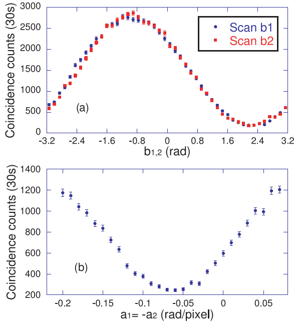
FIG. 3. (Color online) Coincidence counts on a time window of 30 s with the polarizers in front of the couplers set at 45^\circ and -45^\circ . (a) Coincidences as a function of b_1 (blue) and b_2 (red) with b_{2,1} = 0 and optimal a_{1,2} ; (b) coincidences as a function of a_1 = -a_2 with optimal b_1 and b_2 = 0 .
