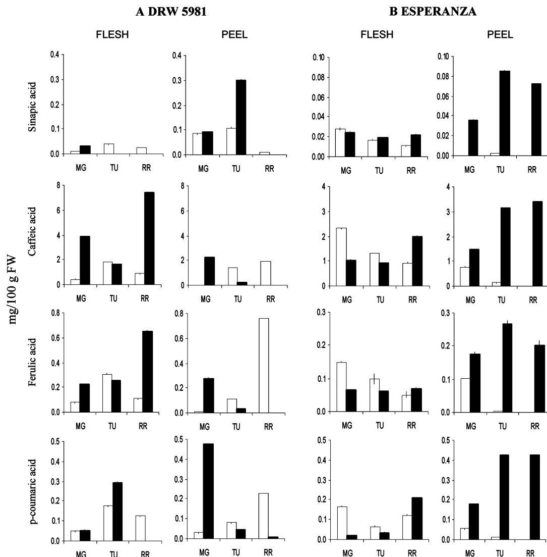
Figure 5. Hydroxycinnamic acid content in flesh and peel of (A) DRW 5981 and (B) Esperanza fruits. Open and solid columns represent control fruits and UV-B-shielded fruits respectively. Data are expressed in milligrams/100 g of fresh weight. Bars represent standard errors of measurements performed in triplicate. Abbreviations: MG, mature green; TU, turning; RR, red ripe.
