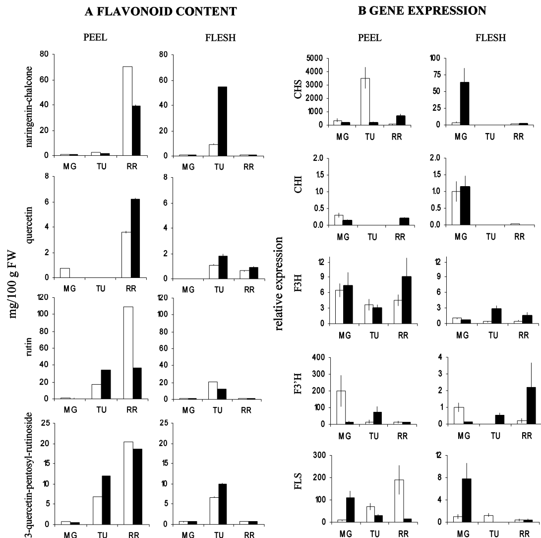
Figure 3. Flavonoid content and mRNA steady-state levels of flavonoid structural genes in flesh and peel of DRW 5981 fruits grown in the presence and deprivation of UV-B. (A) Content of the different flavonoids analyzed in flesh and peel of DRW 5981 cv. Open and solid columns represent control fruits and UV-B-shielded fruits respectively. Data are expressed in milligrams per 100 g of fresh weight. Bars represent standard errors of measurements performed in triplicate. (B) Relative expression levels of CHS , CHI , F3H , F3'H , and FLS structural genes in genotype DRW 5981 with LeEF1 as endogenous control. The transcript amount in the flesh of MG fruits was arbitrarily set to 1 and served as calibrator for relative expression levels in each transcript analysis. Open and solid columns represent control fruits and UV-B-shielded fruits, respectively. Bars represent standard errors of measurements performed in triplicate. Abbreviations: MG, mature green; TU, turning; RR, red ripe.
