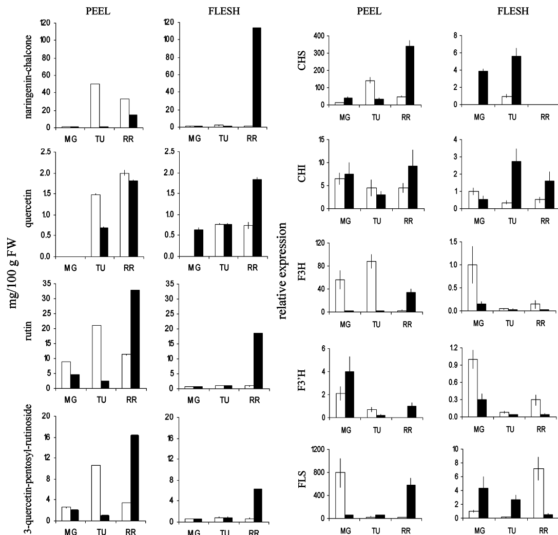
Figure 4. Flavonoid content and mRNA steady-state levels of flavonoid structural genes in flesh and peel of Esperanza fruits grown in the presence and deprivation of UV-B. (A) Content of the different flavonoids analyzed in flesh and peel of Esperanza. Open and solid columns represent control fruits and UV-B-shielded fruits, respectively. Data are expressed in milligrams per 100 g of fresh weight. Bars represent standard errors of measurements performed in triplicate. (B) Relative expression levels of CHS , CHI , F3H , F3'H , and FLS structural genes in genotype Esperanza with LeEF1 as endogenous control. The transcript amount in the flesh of MG fruits was arbitrarily set to 1 and served as calibrator for relative expression levels in each transcript analysis, except in the case of CHS , where its transcript level in the flesh of TU fruit was used as calibrator. Open and solid columns represent control and UV-B-shielded fruits, respectively. Bars represent standard errors of measurements performed in triplicate. Abbreviations: MG, mature green; TU, turning; RR, red ripe.
