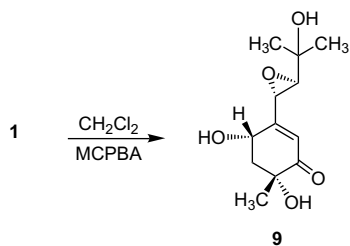
Scheme 2.
