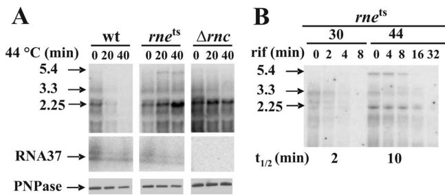
FIG. 5. Stabilization of pnp mRNA and PNPase expression upon RNase E inactivation. Strains C-5869 ( rne + ; wild type [wt]), C-5868 ( rne-3071 ; RNase E-thermosensitive mutant [ rne ts ]), and C-5684 ( Δmcs38::kan ; RNase III-null mutant [ Δrnc ]) were grown at 30°C to an OD 600 of 0.8 and then shifted at 44°C. At different time points from the temperature shift, samples were taken for RNA and protein extraction. Northern and Western blotting were then performed as described in Materials and Methods. (A, upper panels) Northern blotting of a denaturing agarose gel electrophoresis hybridized with radiolabeled PNP5 riboprobe that reveals monocistronic (2.25, arrowhead) and polycistronic (upper bands) pnp mRNAs. (Middle panels) Northern blotting of a denaturing acrylamide gel electrophoresis hybridized with radiolabeled ANTI37 riboprobe that reveals a ladder of PNP37 polyadenylated forms. (Lower panels) Western blotting with anti-PNPase serum as described in Materials and Methods. (B) Decay of C-5686 pnp mRNA at 30 and 44°C. Rifampin (rif) was added to an aliquot of the 30°C culture at an OD 600 of 0.8 and 40 min after the shift at 44°C. Samples were taken at different time points for RNA extractions, and half-lives ( t 1/2 ) were assessed as described. The strain and sample time points after either temperature shift or rifampin addition (in min) are indicated on the figure. The apparent molecular size (in kb) of the major transcripts detected is also shown (see Fig. S1 in the supplemental material). Some variability in the relative intensity of the 2.25- and 5.4-kb mRNAs has been observed with the rne mutant in different experiments.
