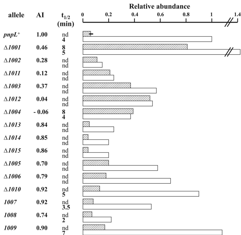
FIG. 4. Relative abundance and stability of \Delta pnp-871 mRNA. Relative abundance and stability were estimated by phosphorimaging quantification of Northern blot signals as described in Materials and Methods. The intensity of all discrete signals has been summed up to evaluate the total abundance of \Delta pnp-871 scar-containing transcript. Data have been normalized to the signals obtained in the pnpL + strain in the absence of PNPase. Data from the pnpL + strain in the presence of PNPase are the average of four experiments, and the error bar is shown. The normalized AI (see text) and half-lives ( t_{1/2} ), when evaluated, are also reported. nd, not determined. Cross-hatched bars, strains harboring pAZ101 expressing PNPase; open bars, strains harboring the empty vector pGZ119HE. In the wild-type C-1a strain (with pnp in a single copy), the half-life is about 1 min (62; unpublished observation).
