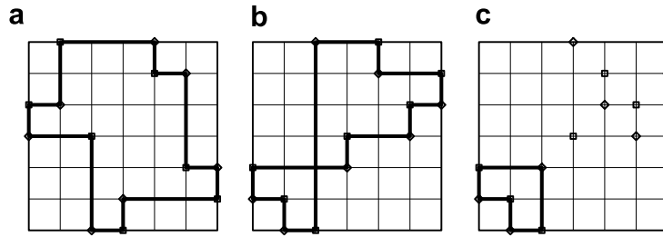
Fig. 2. (a) The permutomino of size n = 7 defined by \sigma = (5,7,4,1,6,3,2) and \tau = (4,5,1,2,7,6,3) (squares represent \sigma , whereas lozenges represent \tau ). (b) The path of \sigma = (3,2,1,4,7,5,6) and \tau = (2,1,7,3,6,4,5) , which does not define a permutomino. (c) The path of \sigma = (3,2,1,4,6,5,7) and \tau = (2,1,3,7,5,4,6) , which does not define a permutomino of size n = 7 .
