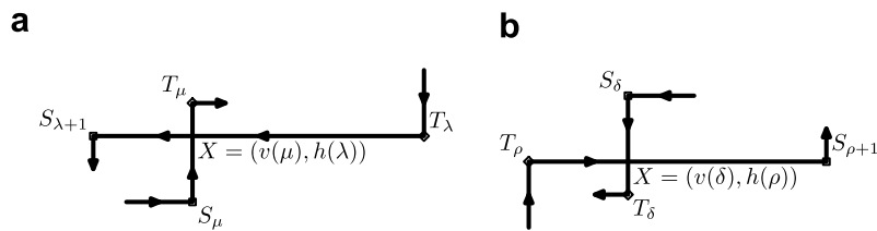
Fig. 6. (a) A UL crossing point at indices (\mu, \lambda) ; (b) A RD crossing point at indices (\delta, \rho) .
