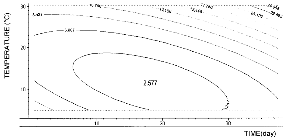
Figure 2. Isoresponse curves for \Delta E as a function of temperature and time at 35% moisture content.
