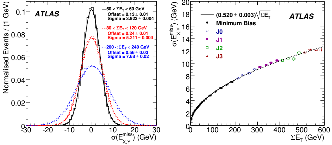
Figure 19: (left) The \cancel{E}_{x,y} resolution for different \Sigma\cancel{E}_T regions in minimum bias events. (right) The \cancel{E}_T resolution in QCD dijet events (J0-J3: see Section 3.1 for definition) is shown together with the \cancel{E}_T resolution from minimum bias events (black filled circles) as a function of \Sigma\cancel{E}_T . An integrated luminosity of the order of 10^{-5} \text{ pb}^{-1} is used.
