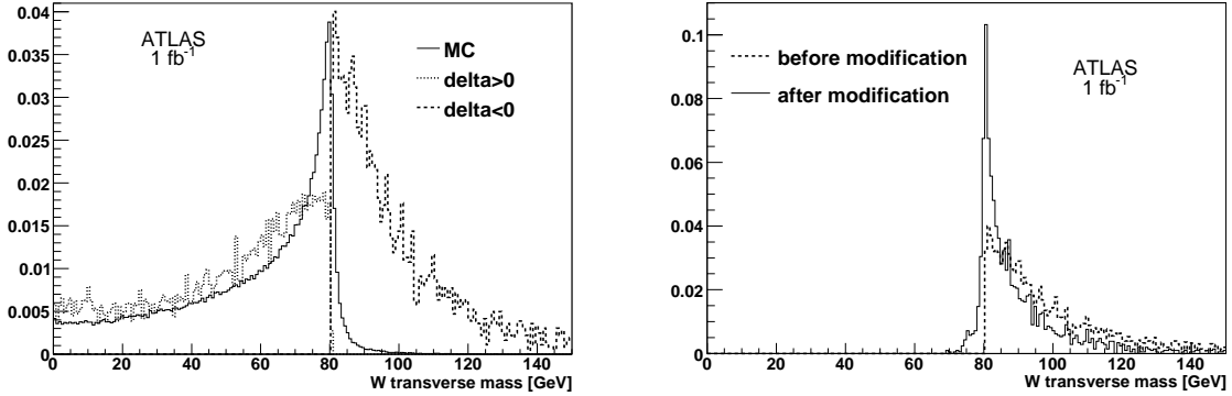
Figure 8: Transverse W boson mass (distributions are normalized to unity). On the left, the Jacobian peak is clearly seen at the generator level (solid line); events for which no p_z^{\nu} solution is found (dashed line) can be distinguished from events for which a solution is found (dotted line). On the right, the effect of the p_T^{\nu} modification for events for which no p_z^{\nu} solution is found, before (dashed line) and after (solid line) modification: a fraction of these events are recovered.
