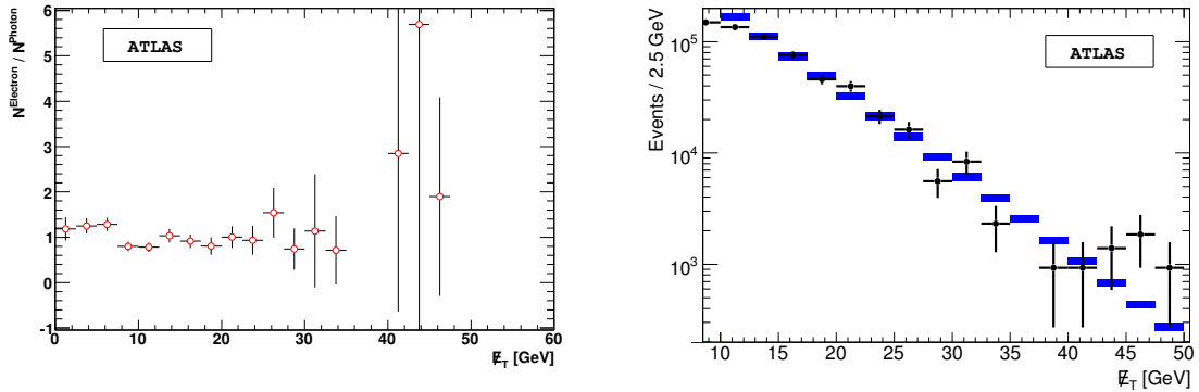
Figure 3: Left: ratio of the \cancel{E}_T distributions in jet background events and in the control sample. Right: comparison of the jet background (points with error bars) and the fitted background (rectangles), for an integrated luminosity of 50 \text{ pb}^{-1} .
