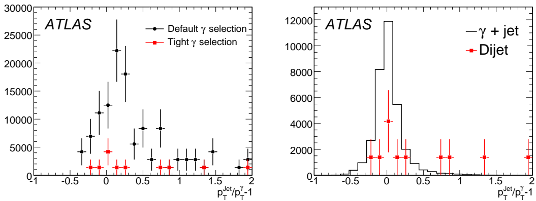
Figure 8: Left: p_T balance for the background sample of 140 < p_T < 280 GeV for the default and tight photon selection. Right: p_T balance for the signal and background sample in the interval 96 < p_{T,\gamma} < 224 GeV for tight photon selection.
