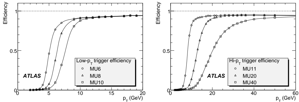
Figure 4: The end-cap trigger efficiency curves for each p_T threshold. The left plot shows the low- p_T thresholds of 6, 8, and 10 GeV and the right plot shows the high- p_T thresholds of 11, 20 and 40 GeV.
