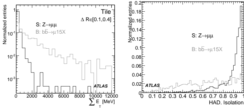
(c) Transverse energy sum in the Tile in the outer ring (d) Isolation variable in Tile calorimeter
