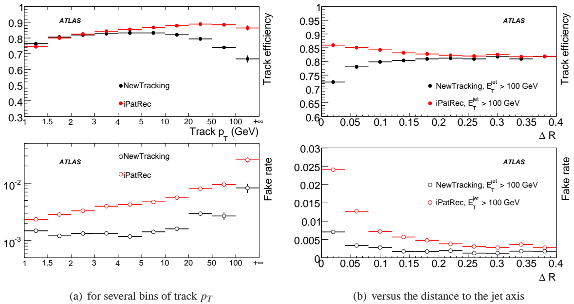
Figure 3: Tracking efficiency (top plots) and fake rate (bottom plots) in t\bar{t} events after the b -tagging quality cuts, for two tracking algorithms: default NewTracking (black symbols) and iPatRec (red symbols).
