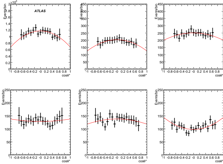
Figure 22: Corrected distributions in polarisation angle \cos\theta^* , for unpolarised Y mesons, in the same slices of Y transverse momentum as in Figure 18. Only \mu\mu\mu 4 sample has been used. Statistics correspond to 10 \text{ pb}^{-1} .
