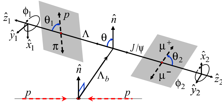
Figure 2: Angles describing the \Lambda_b \rightarrow J/\psi(\mu^+ \mu^-) \Lambda(p \pi^-) decay.
