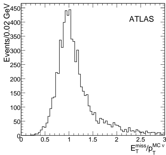
Figure 7: Ratio of \cancel{E}_T to the generated neutrino transverse momentum, after C0 cut. The neutrino considered here is the one from the leptonic W boson decay.
