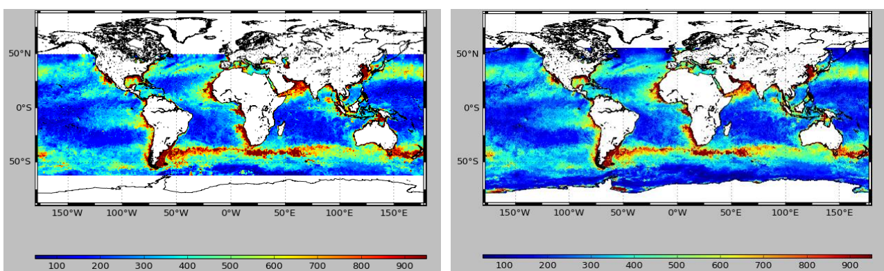
Figure 2: Change in spatial coverage between old and new CMEMS product for the global satellite chlorophyll a (GLOBCOLOR). New product covers the high latitudes but only during spring - summer seasons.
