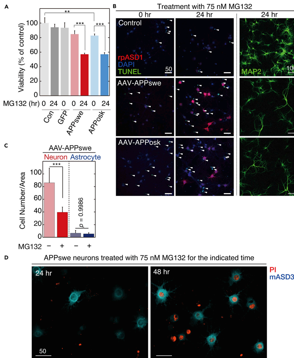
Figure 13. Secreted ASPD Induced Apoptotic Degeneration of Surrounding Neurons
