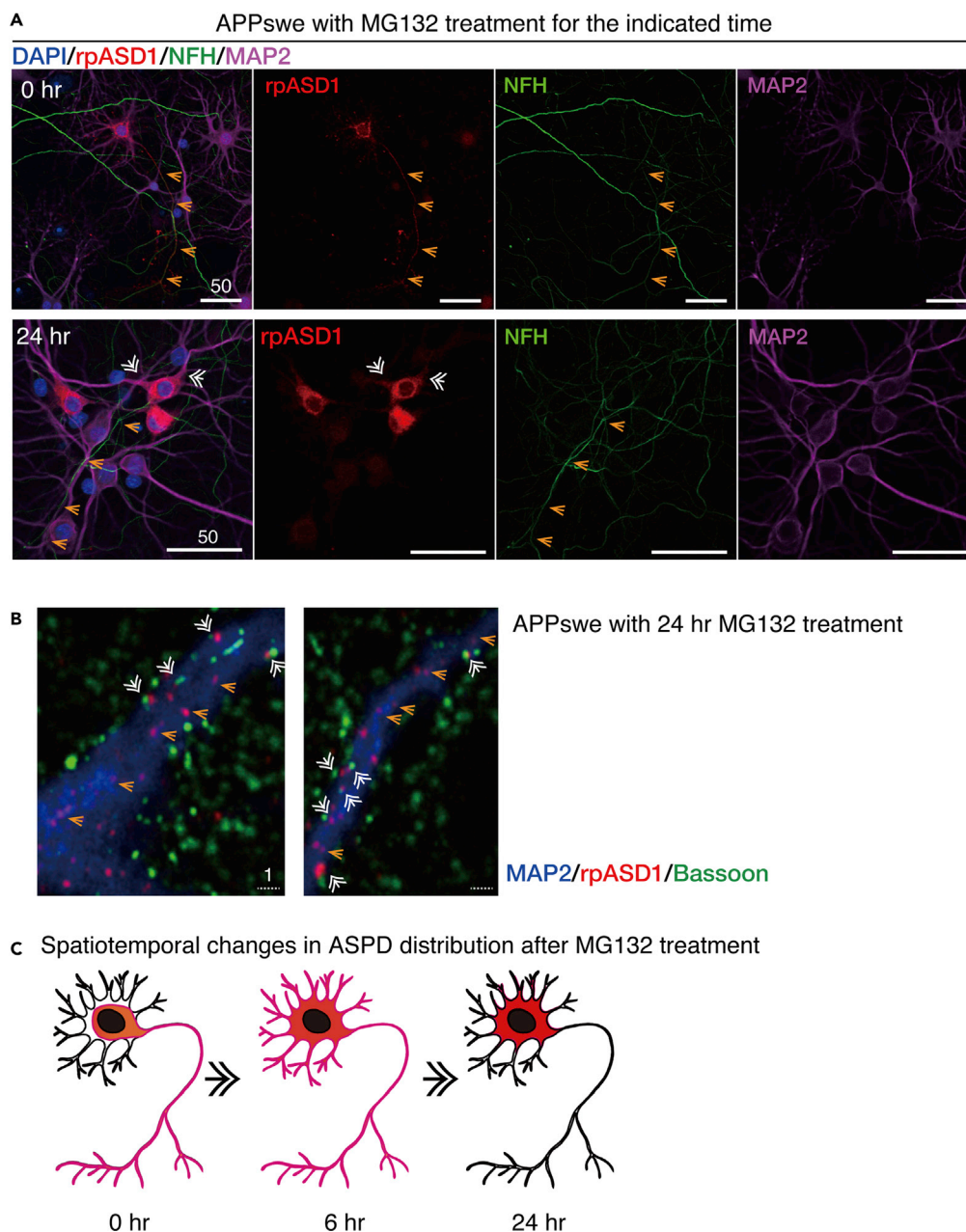
Figure 5. Proteasome Inhibition Changes ASPD Distribution from Axon to Dendrites
