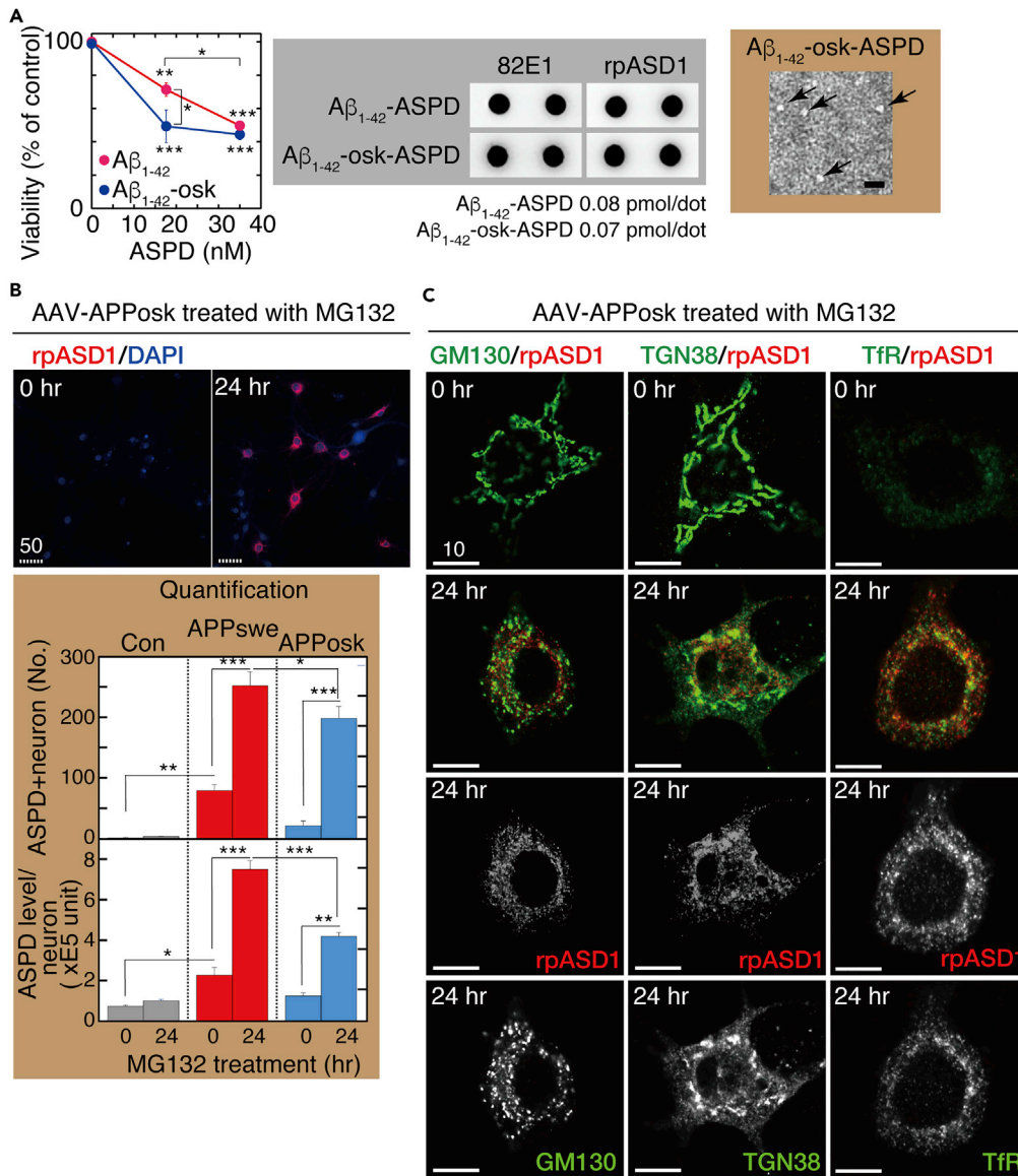
Figure 11. ASPD Form from A \beta_{1-42} -orsk
