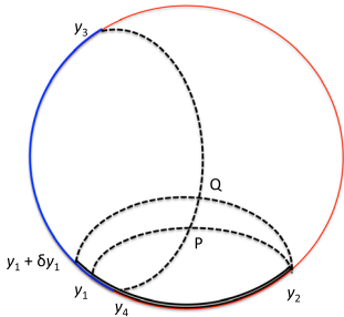
FIG. 3. We have perturbed one of the subregions (from y_1 to y_2 ) by a small amount, so that the new subregion is from y_1 + \delta y_1 to y_2 . It then gives us a different intersection point Q where the bulk field is localized. P and Q are of course, spacelike separated.
