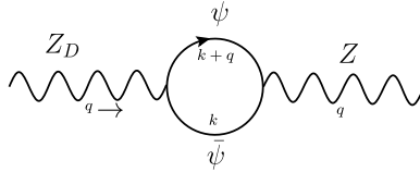
Fig. 8. The mixing between the Z and Z D with the running of ψ particles in the loop.
