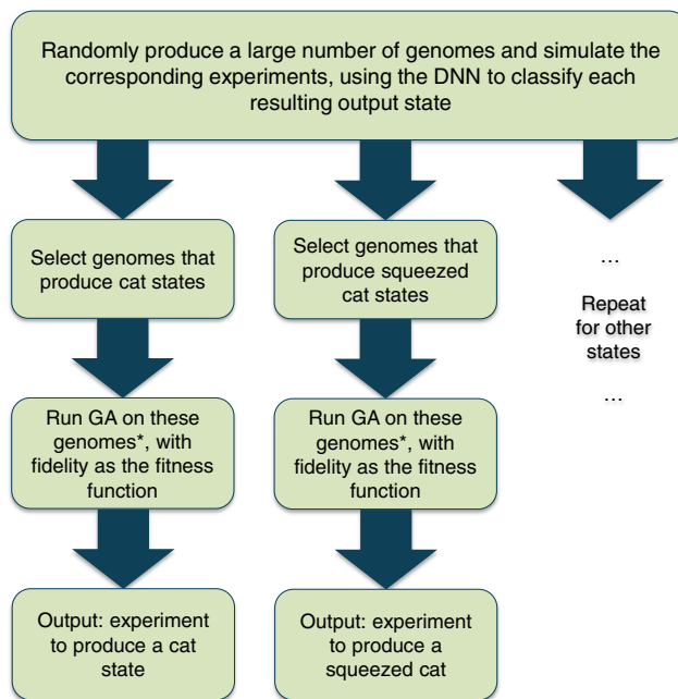
Fig. 4 A flowchart of the overall structure of our hybrid algorithm that incorporates both a deep neural network (DNN) and a genetic algorithm (GA) to design experiments to produce a range of quantum states. *The GA runs in stages 2 and 3 of the 3-stage algorithm discussed in Section 4.1.1 of the main text
