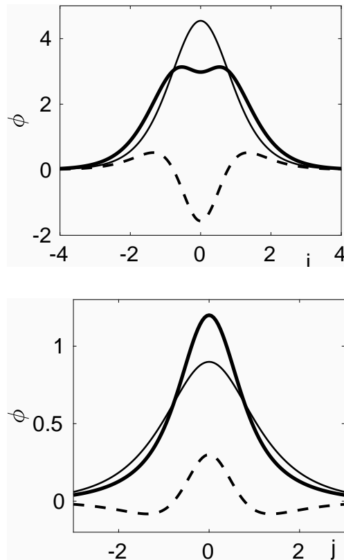
Figure 5. Illustration of the wave-forms for \phi (which is identical to \psi ) for the quadratic case (shown in the upper panel, and corresponds to the parameter values a = 1, b = 0, h = 0.3 ) and the cubic case (shown in the lower panel, given by parameter values a = 0, b = 1, h = 0.2 ), in both cases, C = 1 . In both panels, the thin solid line represents the leading order solution, and the thicker solid line shows the solution including the O(h^2) correction terms, the difference between the two solutions is displayed using thick dashed lines. Note the effect of the different signs in front of the w_{\bar{z}\bar{z}} terms in (4.21) and (5.13). All plots correspond to a mass ratio of \mu = 0.02 .
