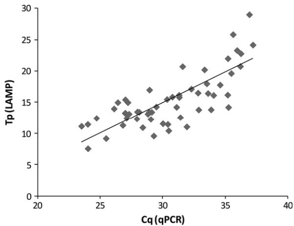
Figure 3 Diagnostic sensitivity of the 23S rRNA LAMP. Time to positive (minutes, Tp) for LAMP and cycles to positive (qPCR, C_q ) are given on y- and x-axis, respectively. Samples with different amounts of FDP (represented with different C_q ) were tested with LAMP assay. Trend line shows a positive correlation ( R^2 = 0.58 ) between Tp and C_q values.
