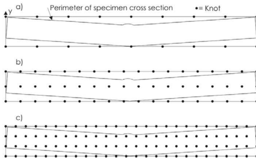
Figure 2-13 Example showing incremental refinement of knots for the smoothing splines. The top (a) shows the coarsest grid, the middle (b) and bottom (c) shows the two next incrementally finer grids [68].
