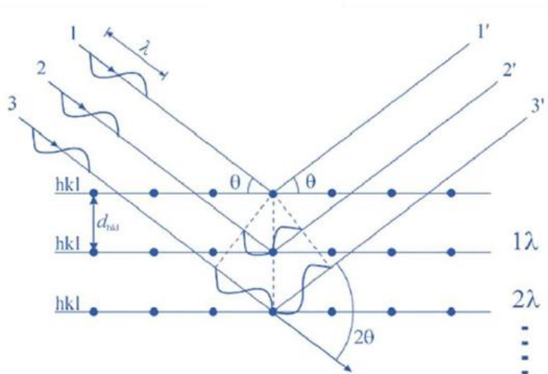
Figure 2-3 Illustration of Bragg's law for diffraction techniques [28]
