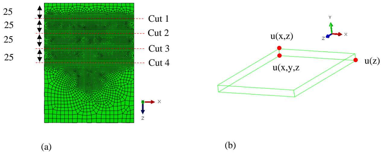
Figure 5-8 (a) XZ view of the FE model of the TG6 used for the simulation of the iCM showing the mesh and location of contour cuts, (b) isometric view of the 3D model showing the BC used during the iCM simulation.
