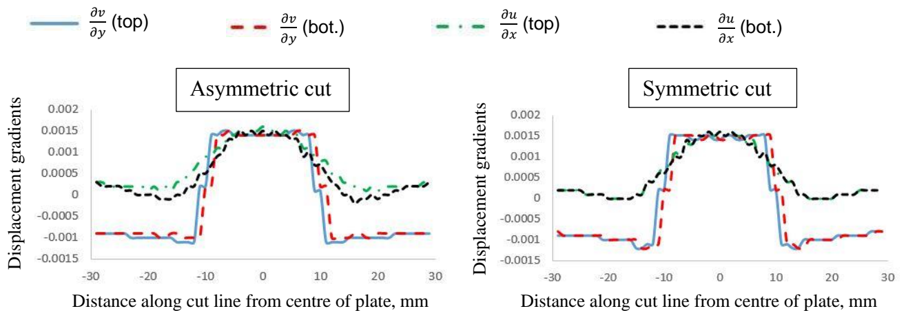
Figure 4-16 (a) Schematic drawing of the composite plate shown on the right. The FE mesh used for the FE modelling is shown on the left together with the location of the contour cut. (b) Comparison of the reconstructed contour stress with the original stress along the measurement line for asymmetric cut shown on the left and for the symmetric cut shown on the right. (c) Comparison of the displacement gradients \frac{\partial v}{\partial y} and \frac{\partial u}{\partial x} on both mating cut surfaces for the asymmetric cut shown on the right and for the symmetric cut shown on the left.
