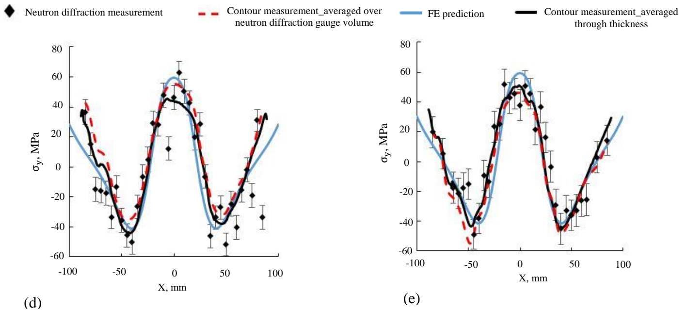
Figure 3-17 Predicted map of the plate (a) with stiffness ratio 1, (b) with stiffness ratio 2 (c), with stiffness ratio 4 (d) line profile of neutron diffraction \sigma_y stress for the plate with stiffness ratio 2 and (e) line profile of neutron diffraction \sigma_y stress for the plate with stiffness ratio 4. Also shown in (d) and (e) are line profiles of FE predicted transverse stress and measured transverse stress for asymmetric cuts using the contour method. The experimental data is discussed later in the thesis.
