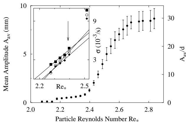
FIG. 6. The mean amplitude (left ordinate in millimeters, right ordinate in units of the grain size) as a function of the shear stress. The error bars denote the standard deviation. The inset shows the behavior of the growth rates for modes 8 ( \circ ), 10 ( \square ), and 13 ( \blacklozenge ). The arrow indicates the upper data points included in the linear fit.
