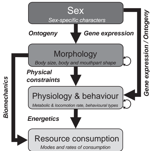
Figure 1. Hierarchical framework for organising the phenotypic traits controlling resource consumption. Each box represents a type of traits (examples are given in italics). Examples of biological mechanisms and processes underpinning causal relationships (arrows) are given in bold italics. Two-headed arrows represent covariations between traits of the same type.
