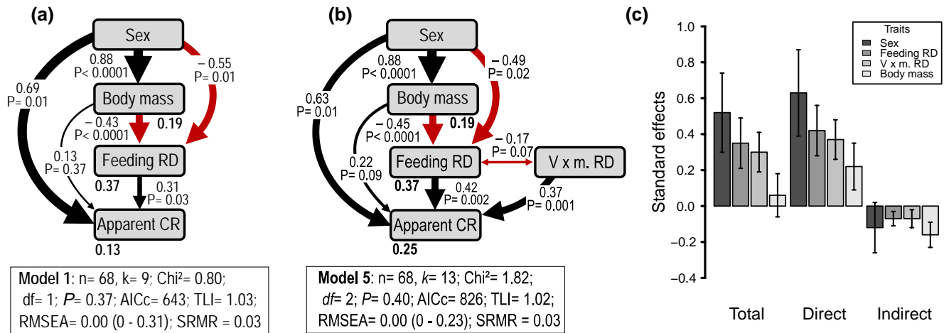
Figure 4. (a) Initial structural equation model describing how a behavioural trait (Feeding RD) constrains the effects of body mass and sex on apparent consumption rate of litter. (b) Final structural equation model including a physiological trait used as a proxy of specific metabolism in activity ('V × m. RD'). Black and red arrows indicate positive and negative relationships, respectively, and the size of arrows is proportional to path coefficients (i.e. beta estimates). The signs of path coefficients of 'Sex' correspond to the effect of male compared to that of female gammarids. The two-headed arrow represents covariances. r^2 -values are given in bold. The boxes below the models contain summary statistics. A valid model should have a \chi^2 p-value > 0.05, RMSEA < 0.06, TLI > 0.90 and SRMR < 0.08. (c) Barplots of total, direct and indirect effects assessed in the final model shown in panel (b). Error bars are standard errors (SE).
