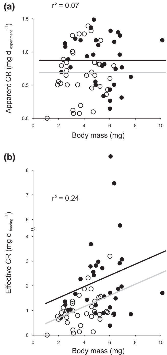
Figure 3. Apparent (a) and effective (b) consumption rate of litter by gammarids as a function of body mass. Solid and open dots depict males and females, respectively. Black and grey lines are intercepts (a) and regression lines (b) for males and females, respectively. r^2 -values are computed from a model including body mass and sex as main effects.
