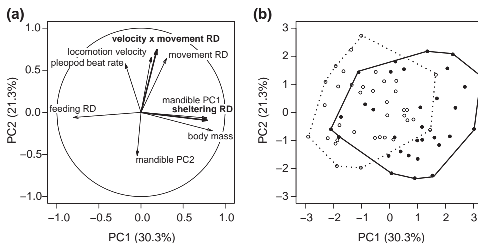
Figure 2. Principal component analysis of phenotypic traits. The correlation circle (a) and ordination plot of the individuals (b) were drawn for the two first principal components, which condensed 51.6% of the total variation in phenotypic traits within the dataset. Traits in regular characters were specified as active variable and those in bold characters were included as supplementary variables (a). Solid and open dots depict males and females, respectively (b). The convex hull of all individuals of the same sex is also displayed.
