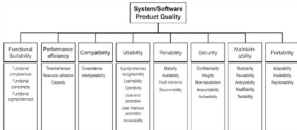
Fig. 1. Software Quality Model based on ISO/IEC25010 [30]
