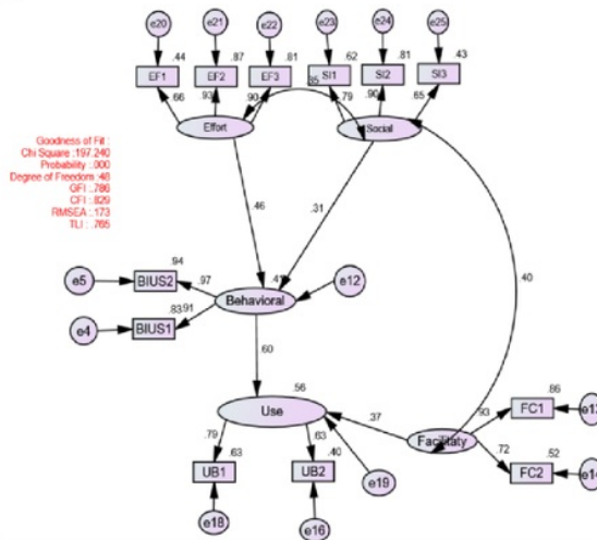
Figure 3 Output Path Diagram Initial Modification
