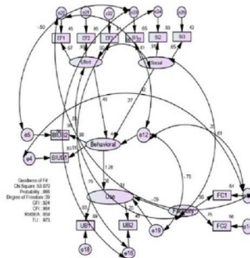
Figure 4. Output Path Diagram Latest Modification
