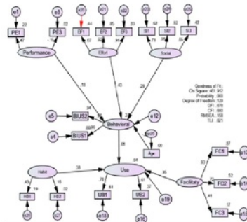
Figure 1. Output Path Diagram Initial Model
