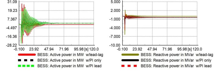
Fig. 16. BESS active and reactive power
