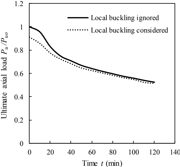
Fig. 20. Influences of local buckling on the ultimate axial strength of CFST column subjected to various time exposure to fire.
