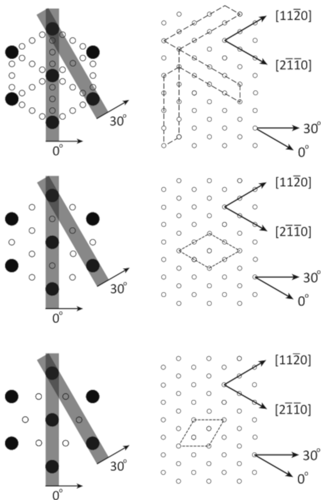
Fig. 2. Interpretation of RHEED periodicities for CrSb(0001), with reciprocal space on the left and real space meshes on the right. Shaded regions represent the regions of reciprocal space accessed by RHEED. From top to bottom are shown (1 \times 4) , (2 \times 2) , and (\sqrt{3} \times \sqrt{3})R30^\circ .
