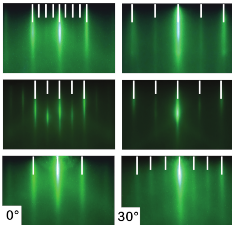
Fig. 1. RHEED patterns in two azimuths (defined in Fig. 2) for three surface reconstructions of \text{CrSb}(0001) : \text{td}(1 \times 4) [top], (2 \times 2) [middle], and (\sqrt{3} \times \sqrt{3})R30^\circ [bottom]. Longer white dashes highlight integer order streaks, with fractional orders shown by shorter dashes.
