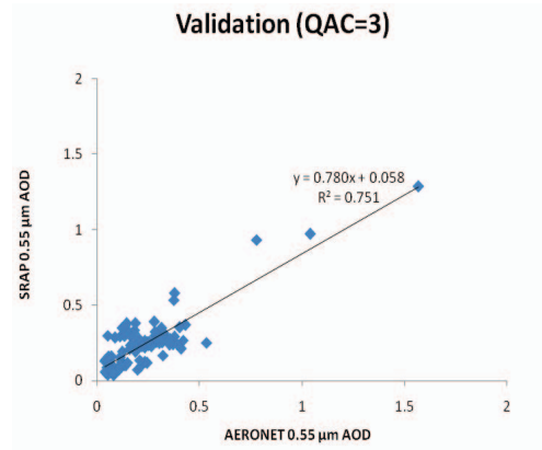
Fig. 4. Comparison between AOD of QAC = 3 and AERONET data
