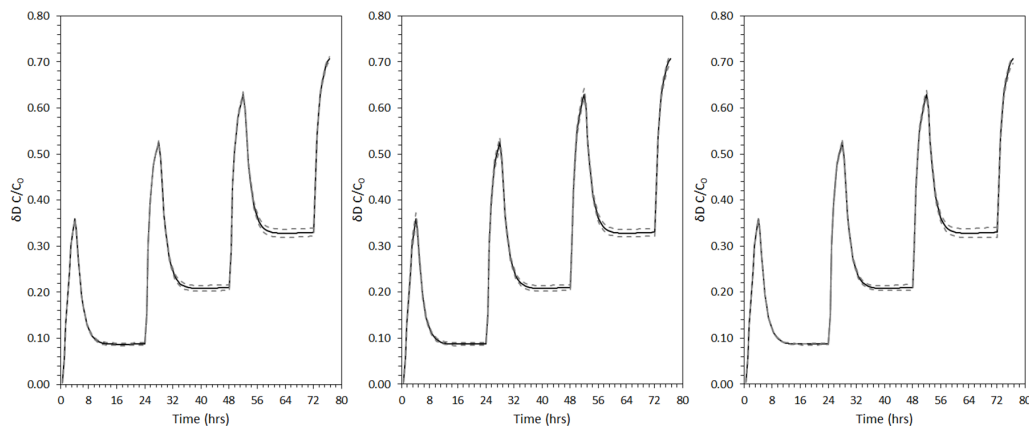
Figure 5. Sensitivity of the dual domain model for the core sample taken from 5.03 m b.g.l. for the calculated error associated with the constrained parameters: \varnothing (LHS); L_c (middle), and \mu (RHS).
