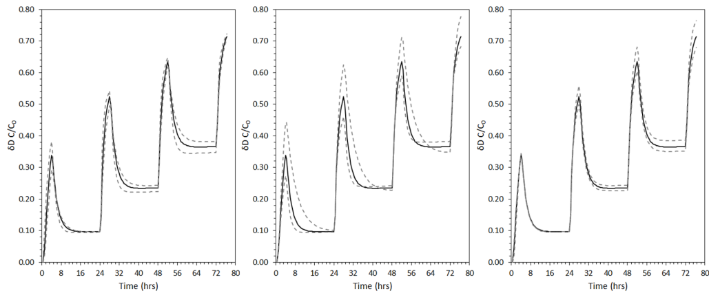
Figure 4. Sensitivity of the dual domain model for the core sample taken from 5.03 m b.g.l. due to \pm 50\% change in unconstrained parameters: \varnothing_m (LHS), \gamma (middle), and \alpha (RHS).
