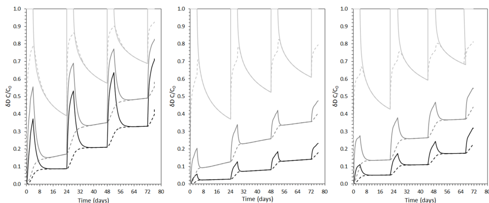
Figure 3. Model output for mobile (solid lines) and immobile (dashed lines) domains for core samples taken from 5.03 m (left), 9.52 m (middle), and 21.75 m b.g.l. (right). The black, dark grey, and light grey lines comprise model output for the base, middle, and top of the cores, respectively.
