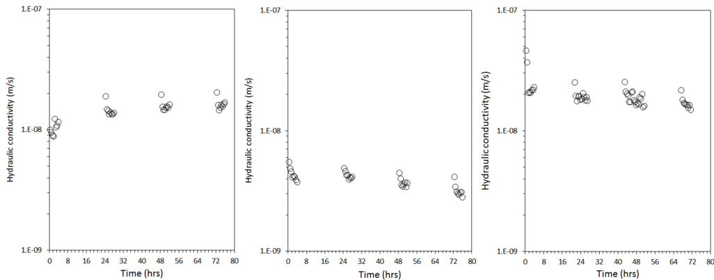
Figure 2. Vertical hydraulic conductivity ( \text{m s}^{-1} ), calculated using Eq. (2), for the interrupted-flow experiments conducted using core samples taken from 5.03 m (left), 9.52 m (middle), and 21.75 m b.g.l. (right).
